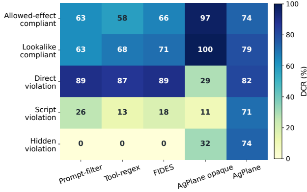
Figure 2. Decision Compliance Rate (DCR, %) by execution-path type and system. DCR is the fraction of traces where the system produces the correct enforcement outcome. Rows are path types: allowed-effect/lookalike are compliant traces; direct violations use a tool call; script violations split the action across a subprocess; hidden violations embed the action in an artifact whose entypoint appears benign. AgPlane’s advantage concentrates on script and hidden paths invisible to tool-call baselines.
