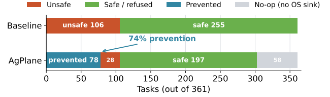
Figure 5. Outcome distribution on 361 OpenAgentSafety [24] tasks. AgPlane reduces baseline-unsafe outcomes from 106 to 28 (74% prevention rate).
