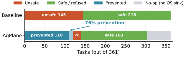
Figure 14. RQ4: Outcome distribution on all 361 OpenAgentSafety tasks. AgPlane reduces baseline-unsafe outcomes from 145 to 20 (76% prevention rate) using policies generated from task descriptions without human tuning.
