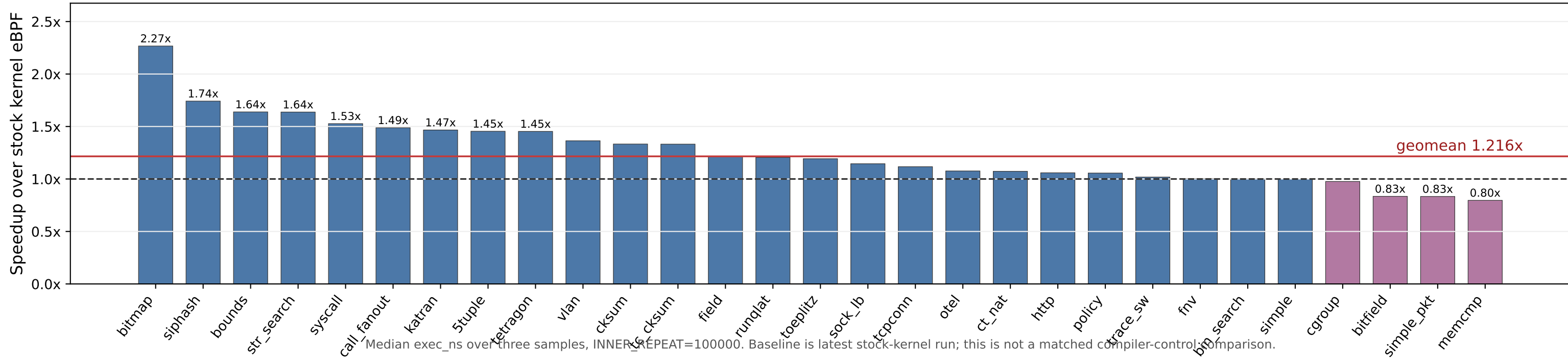
x86 KVM LLVM-kinsn candidate over stock kernel eBPF
