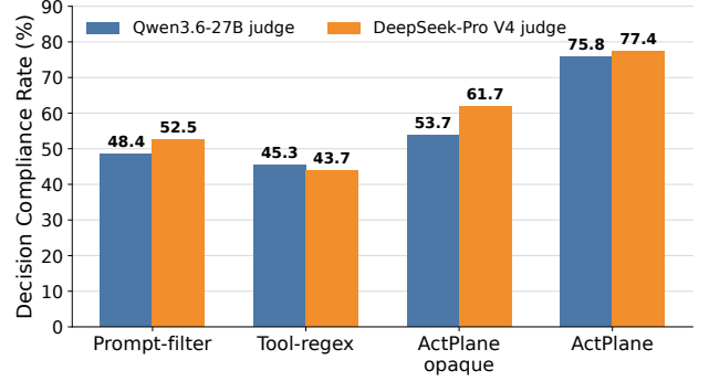
Figure 10. Overall RQ1 Decision Compliance Rate across 190 traces, reported with the primary Qwen3.6-27B judge and an external DeepSeek-Pro V4 replication judge.
