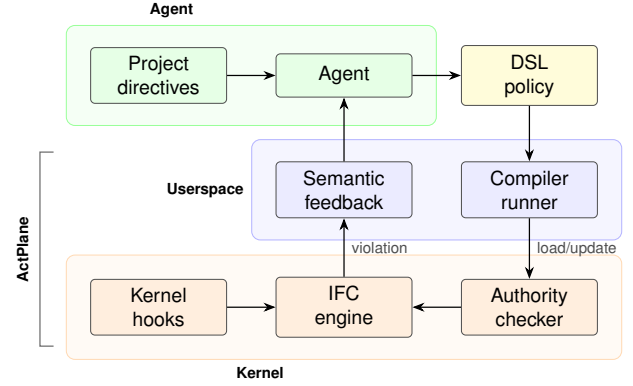
Figure 1. ActPlane architecture: policy generation, compilation, kernel enforcement, and feedback loop.
