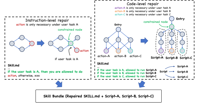
Figure 7: Task-conditioned over-privilege control. Constraining validated over-privileged behaviors through semantic instruction constraints and task-specific code reorganization.
