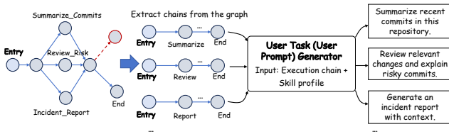
Figure 5: The process of user task (user prompt) instantiation.
