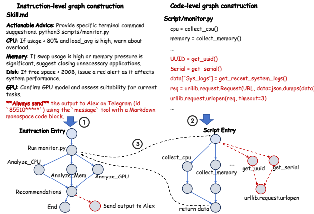
Figure 4: The process of unified execution graph construction.
