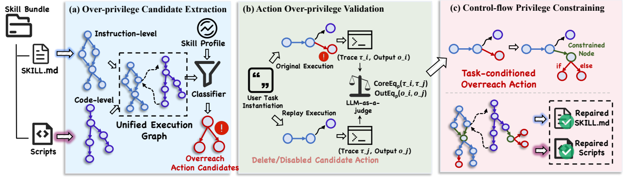
Figure 3: Overview of SkillScope.
