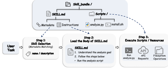
Figure 1: Progressive disclosure in Agent Skill execution.
