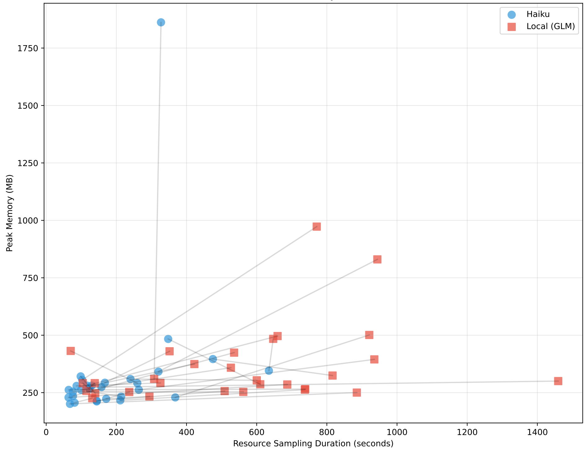
Duration vs Peak Memory (Haiku vs Local)
