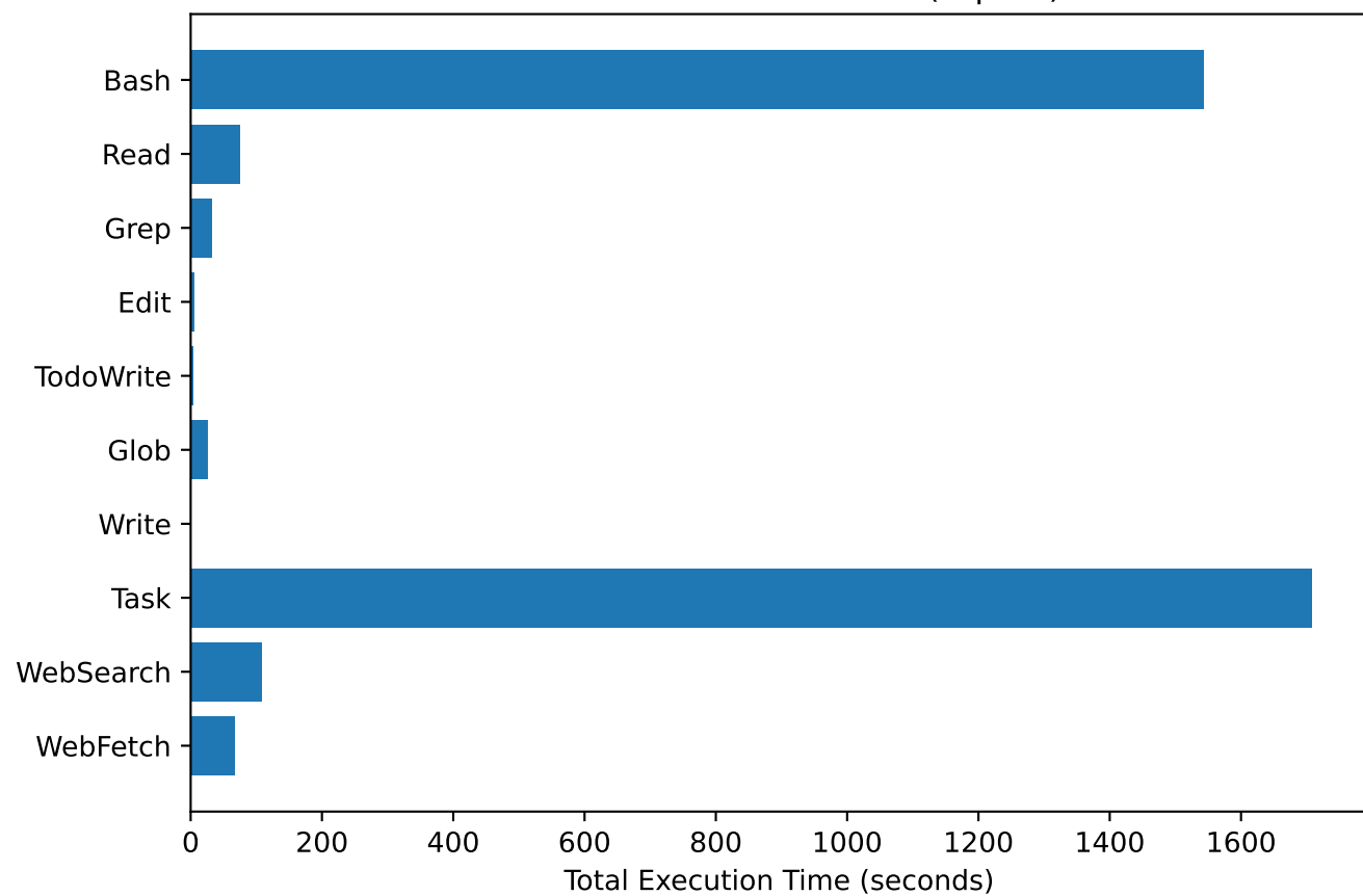
Tool Execution Time Distribution
