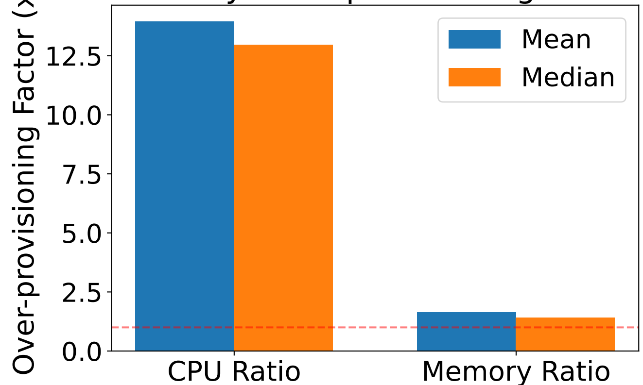
Summary: Over-provisioning Factors
