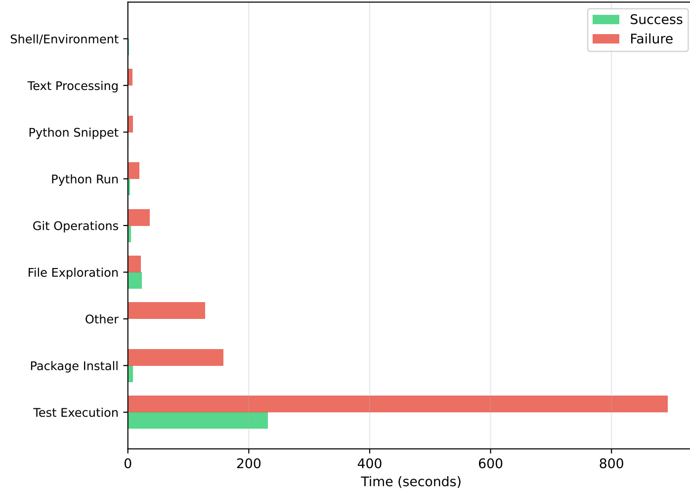
Bash Category Time: Success vs Failure
