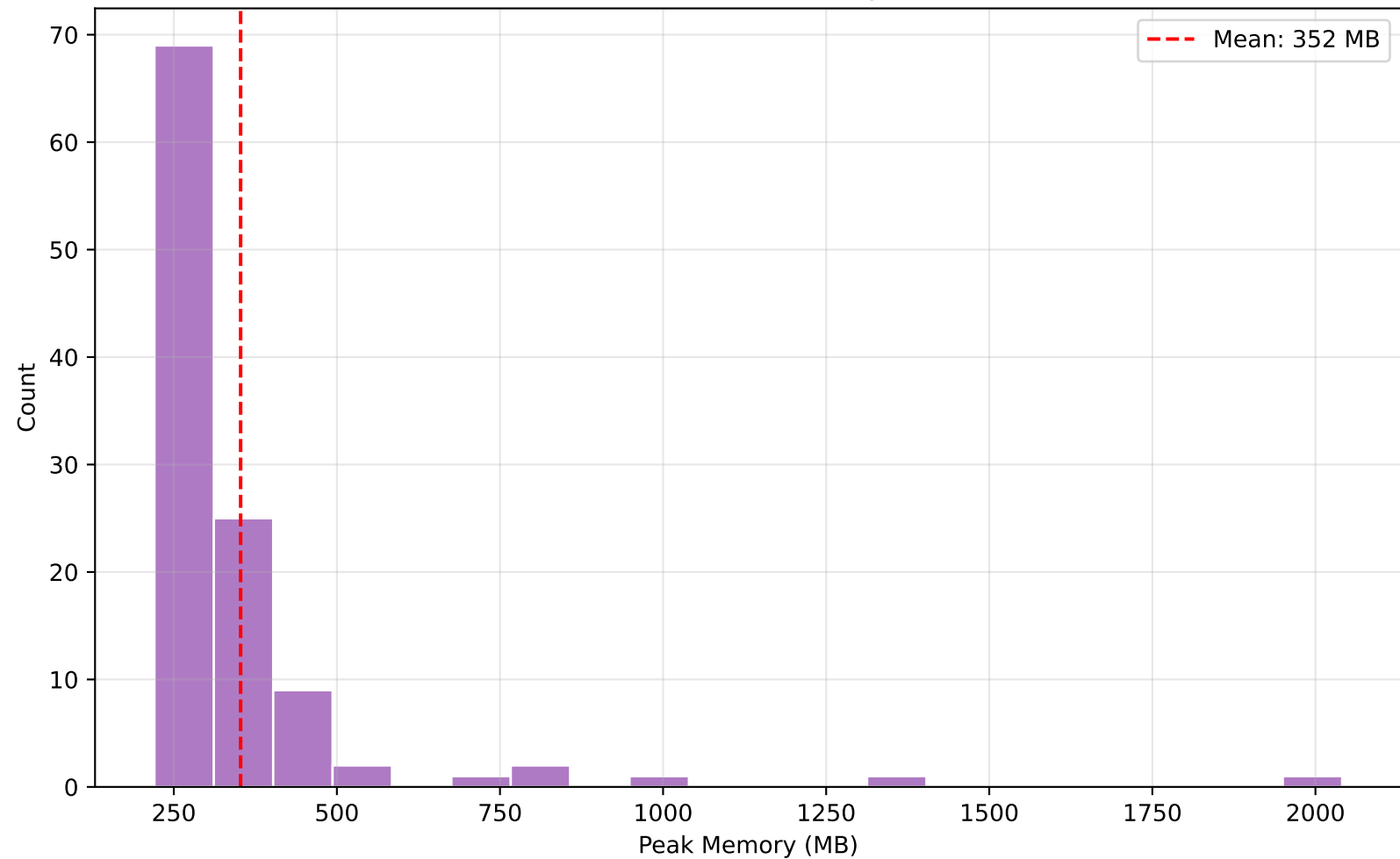
RQ2: Domain Mismatch - Peak Memory Distribution (Local)
