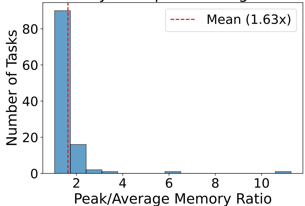
Summary: Over-provisioning Factors
