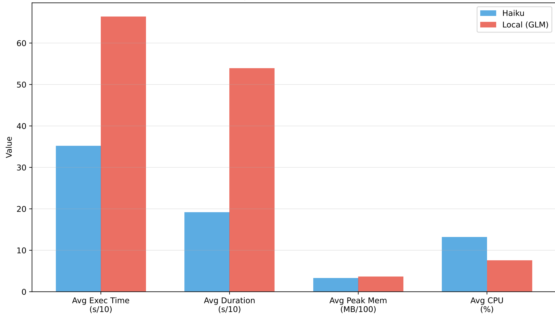
Overall Comparison: Haiku vs Local (30 tasks)
