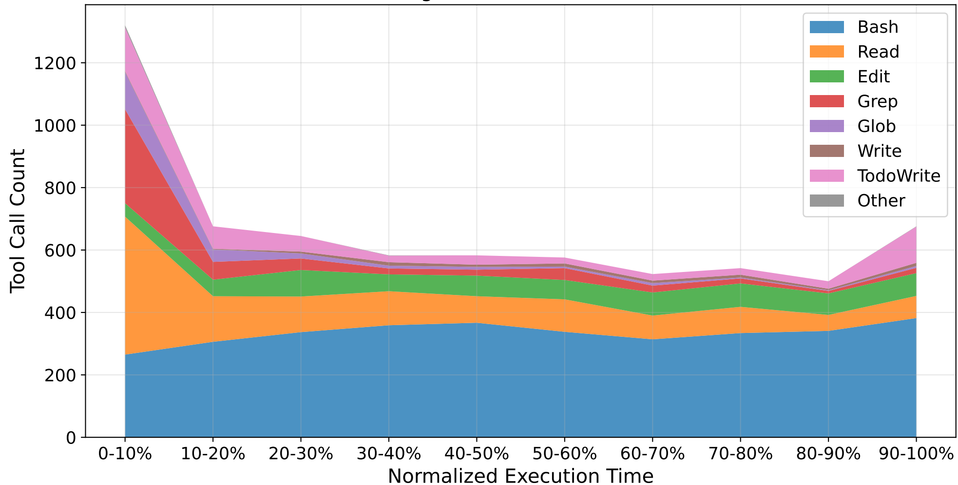
Tool Usage Over Execution Timeline
