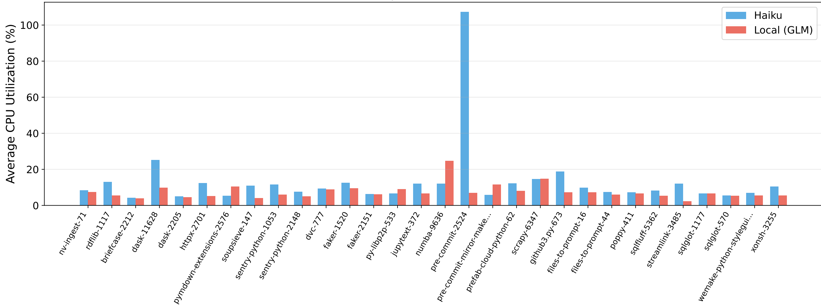
CPU Utilization Comparison: Haiku vs Local (30 tasks)
