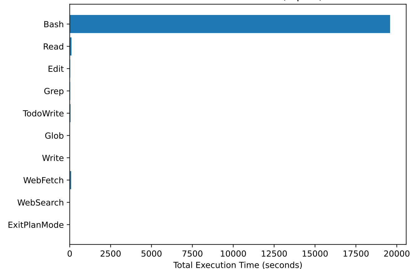
Tool Execution Time Distribution
