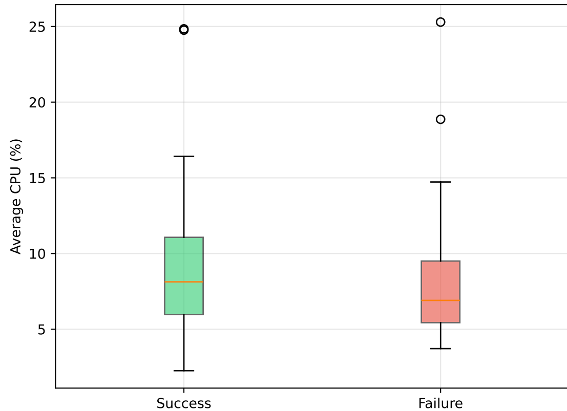
CPU Utilization
