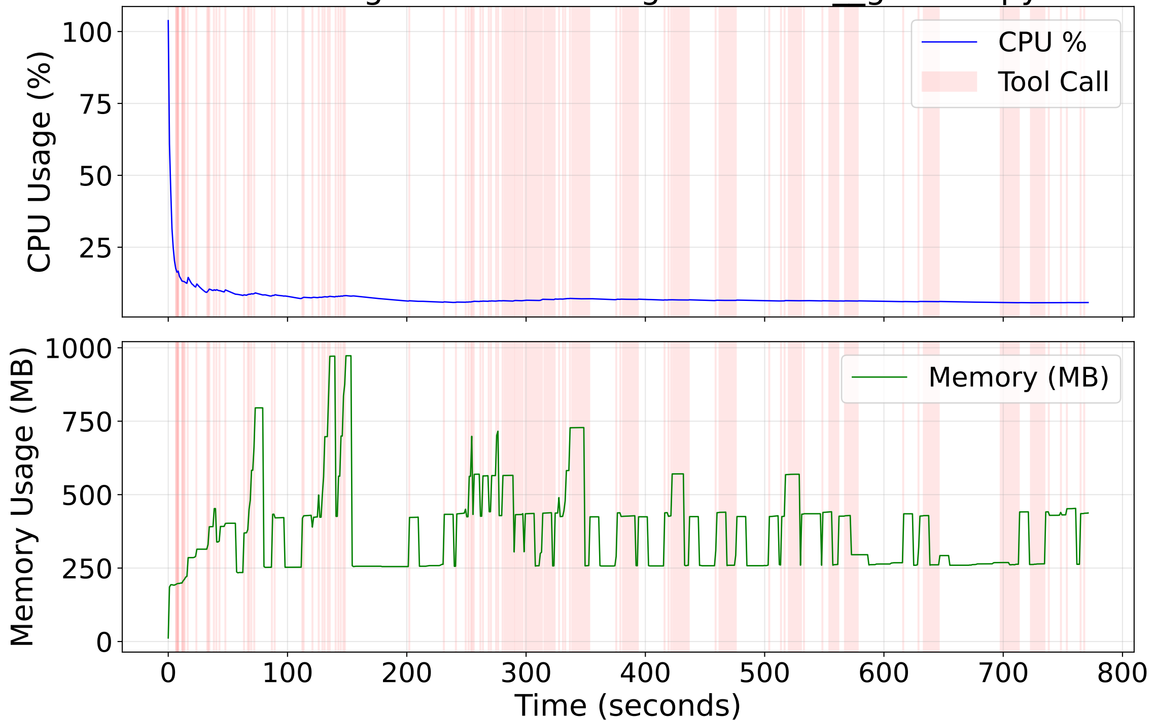
Resource Usage Over Time - sigmavirus24_github3.py-673
