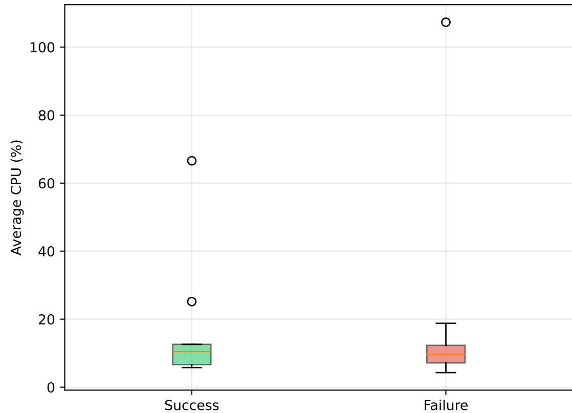
CPU Utilization
