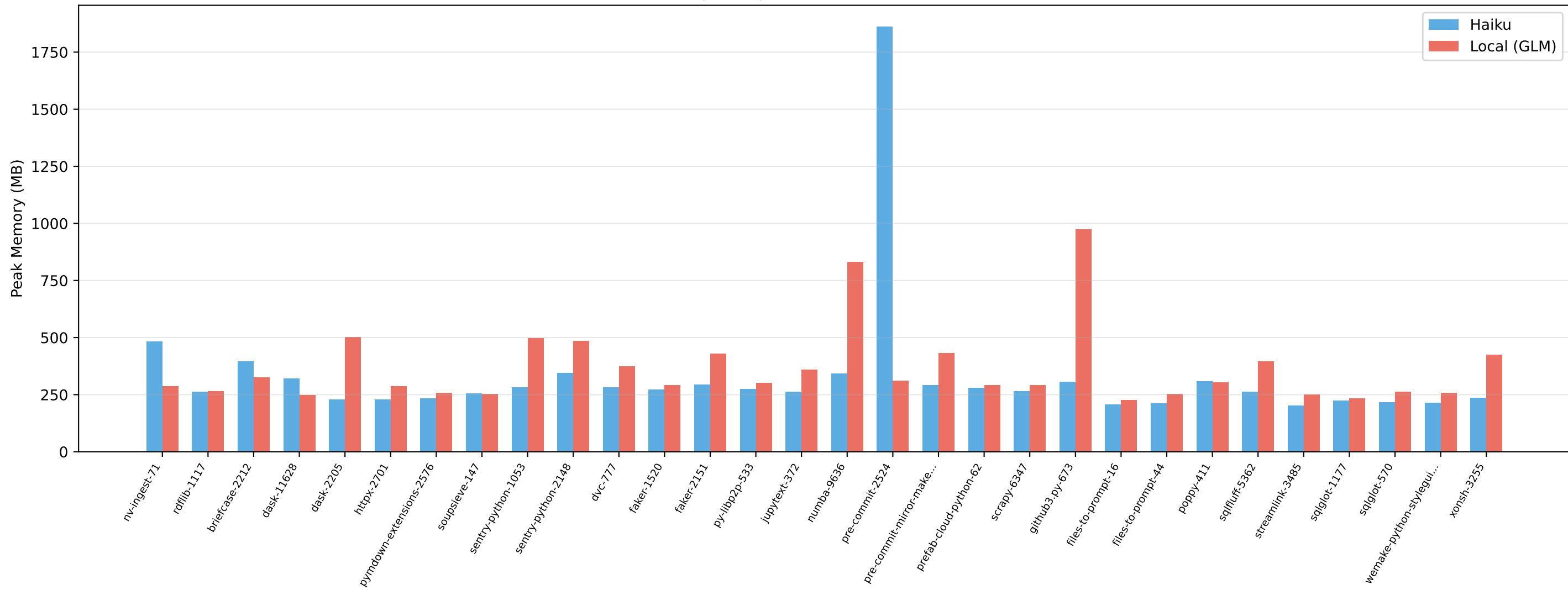
Peak Memory Comparison: Haiku vs Local (30 tasks)
