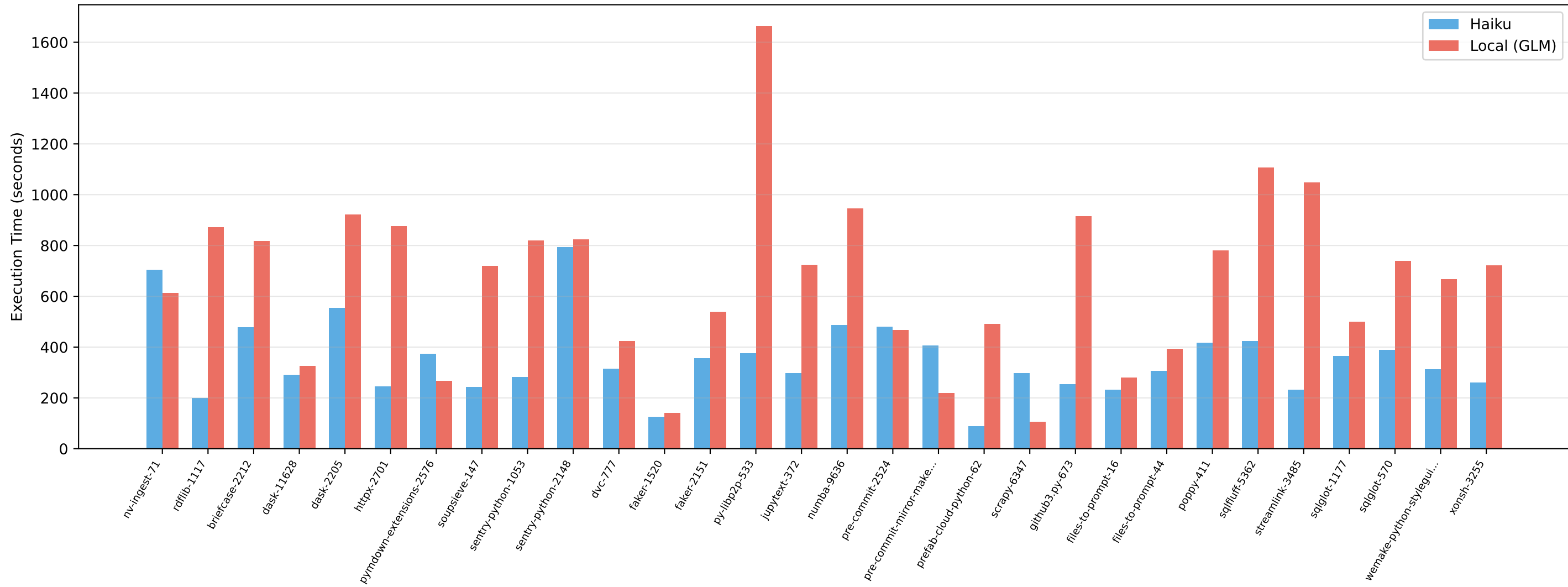
Execution Time Comparison: Haiku vs Local (30 tasks)
