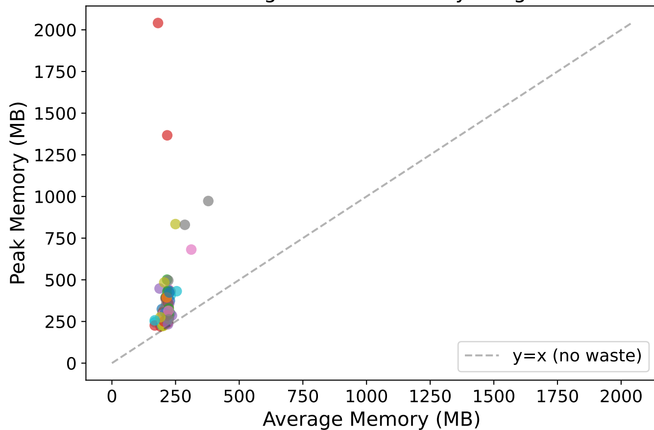
Average vs Peak Memory Usage
