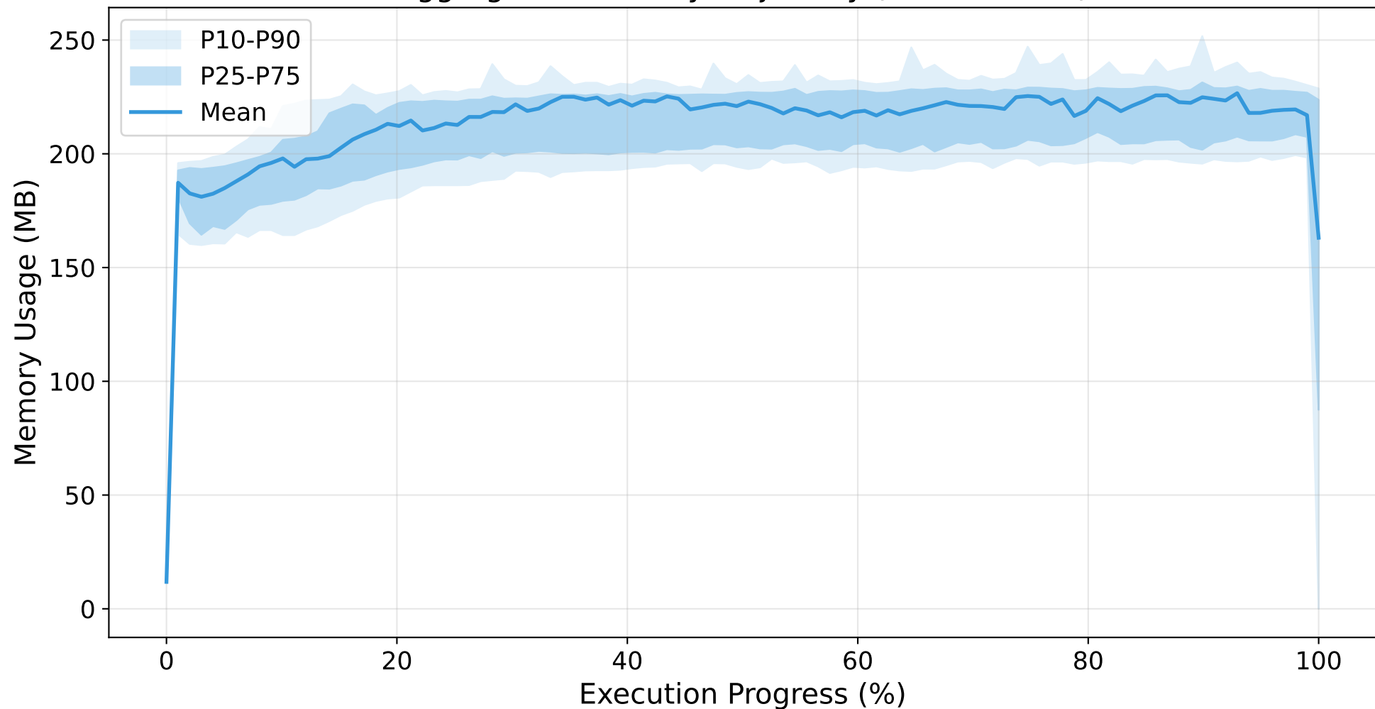
Aggregated Memory Trajectory (n=111 tasks)
