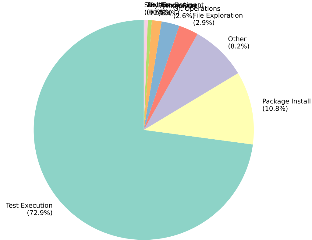
Bash Time by Category
