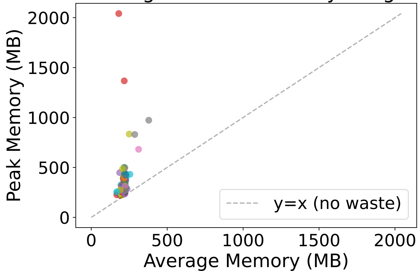
Average vs Peak Memory Usage
