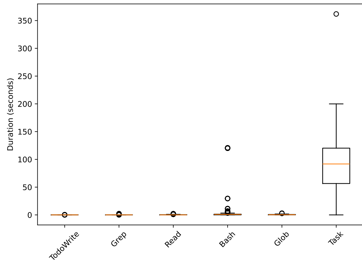
Tool Execution Time Distribution
