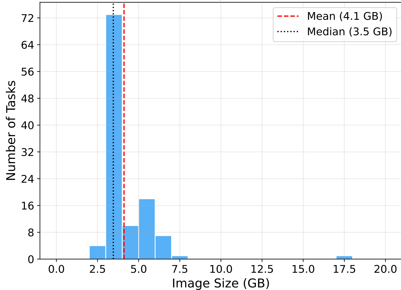
(a) Docker Image Size (n=114)
