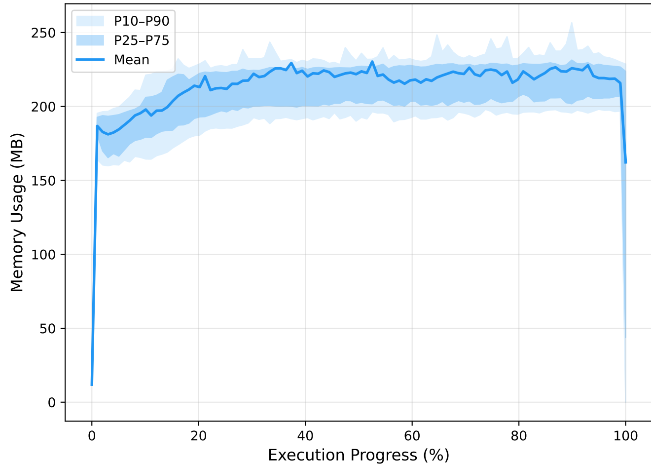
(b) Aggregated Memory Trajectory (n=114 tasks)
