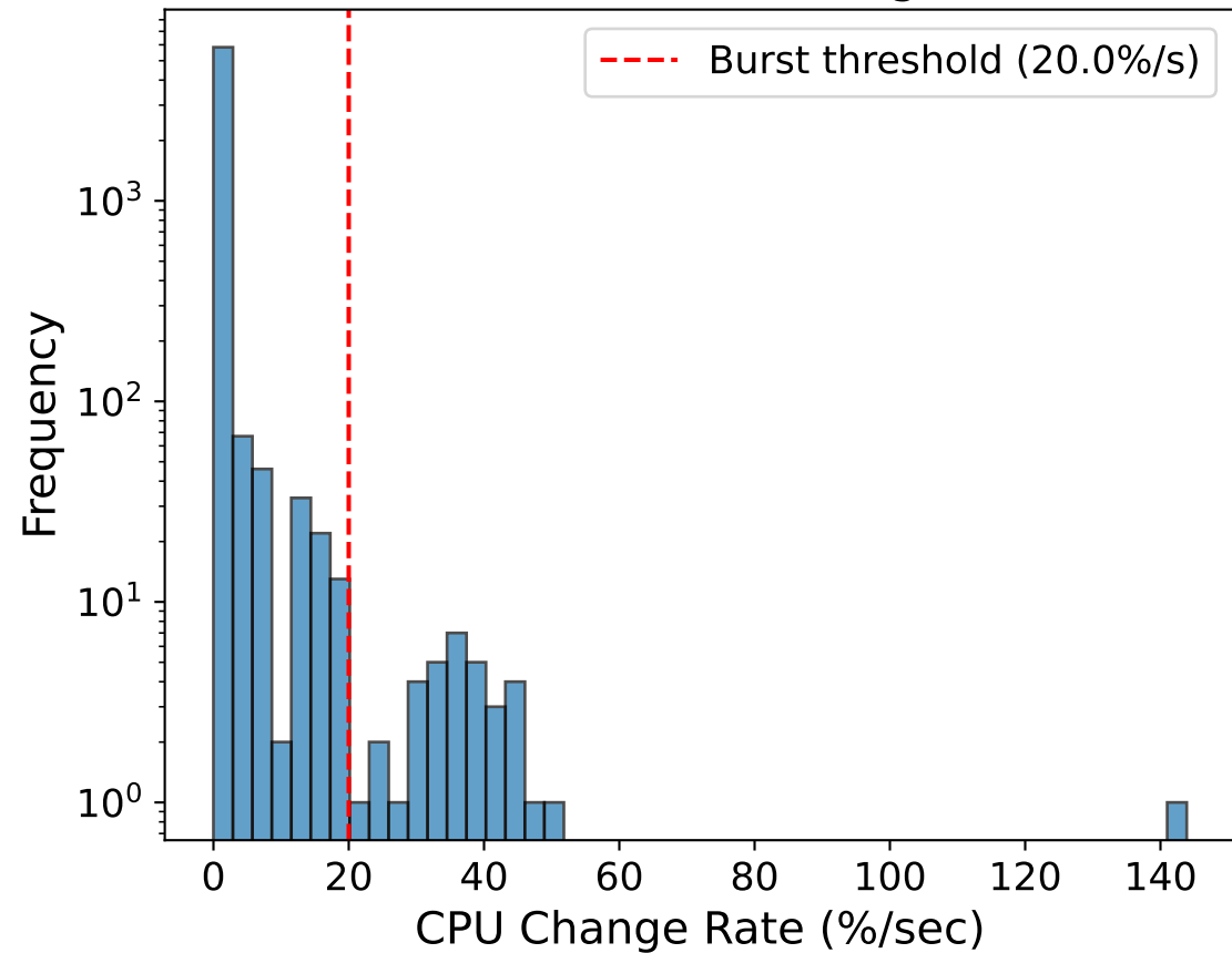
Distribution of CPU Change Rates
