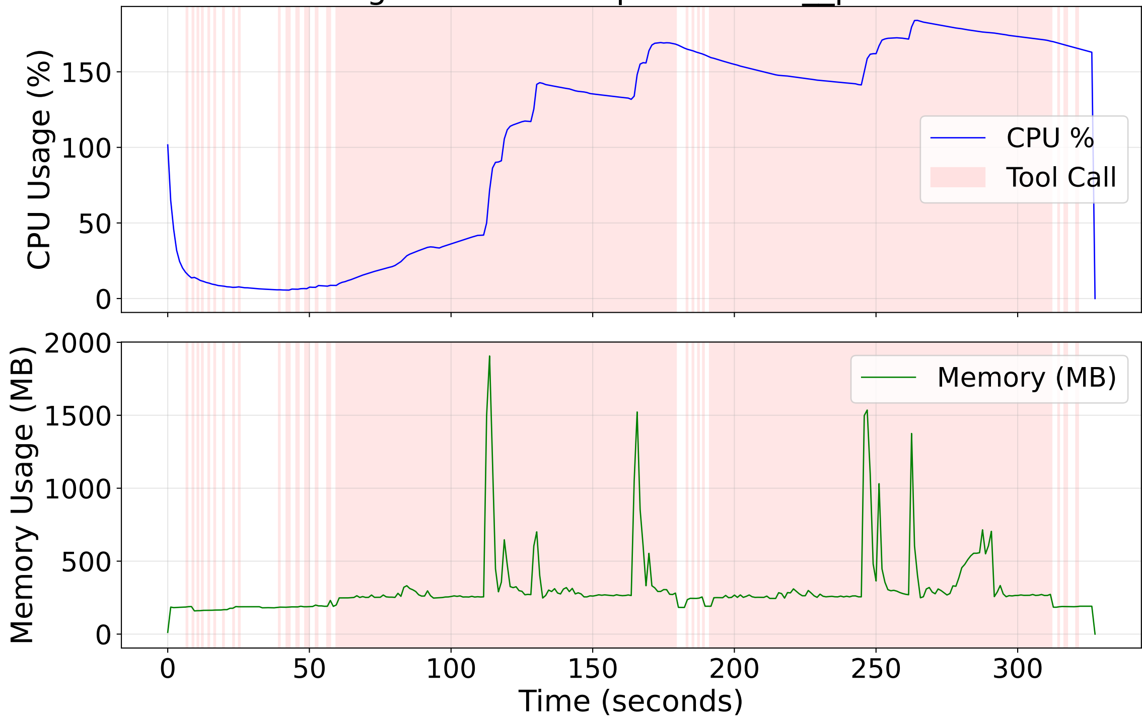
Resource Usage Over Time - pre-commit_pre-commit-2524
