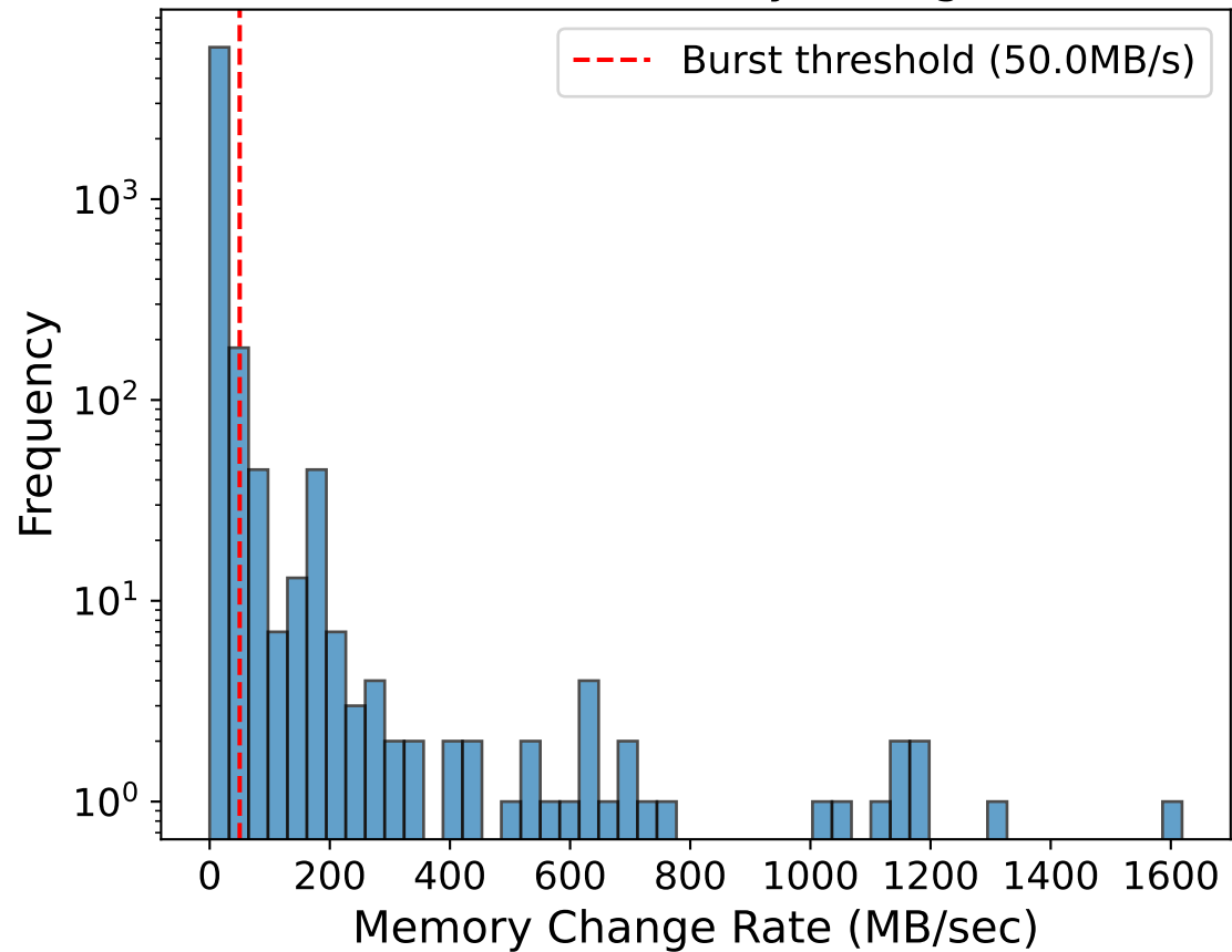
Distribution of Memory Change Rates
