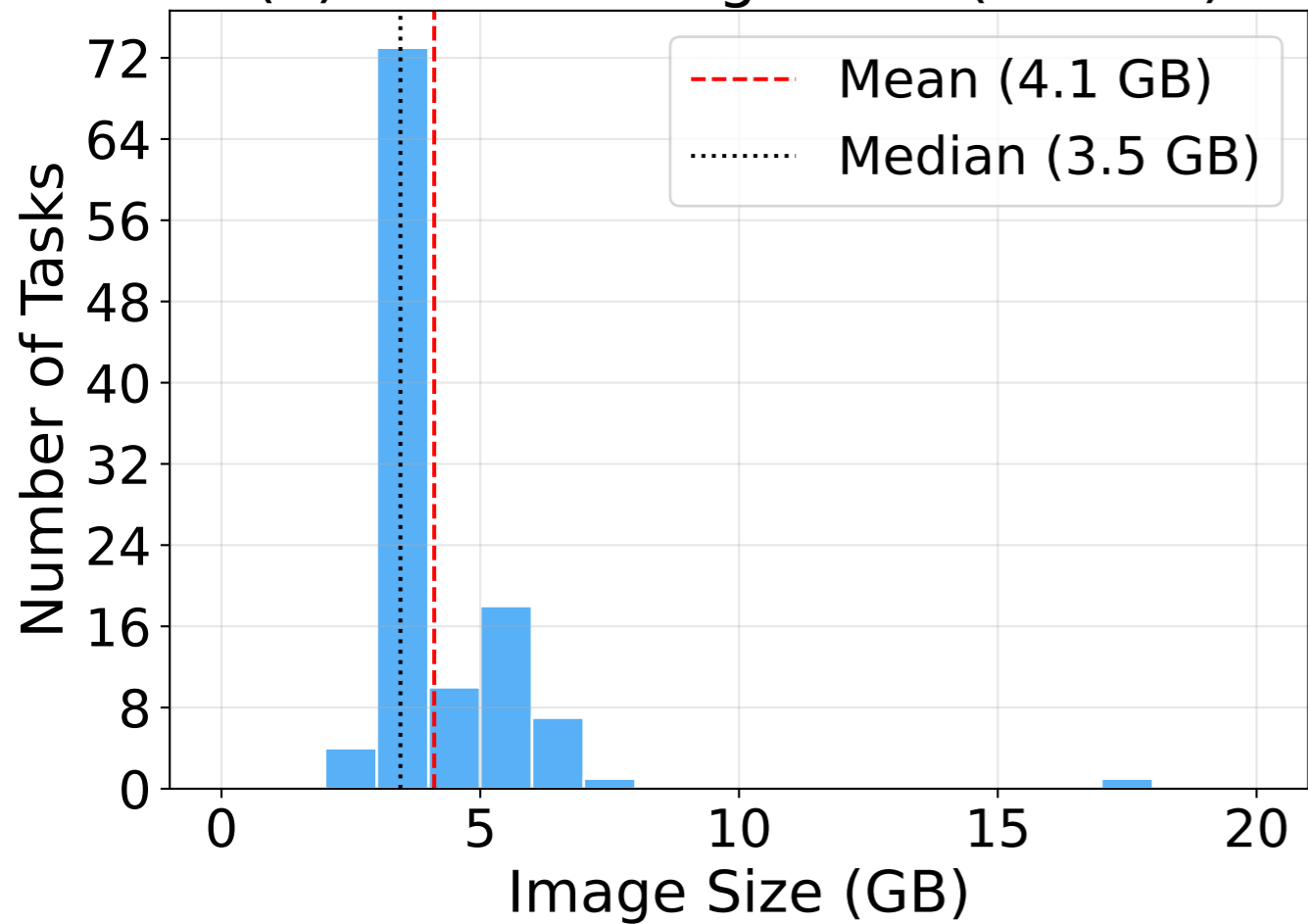
(a) Docker Image Size (n=114)
