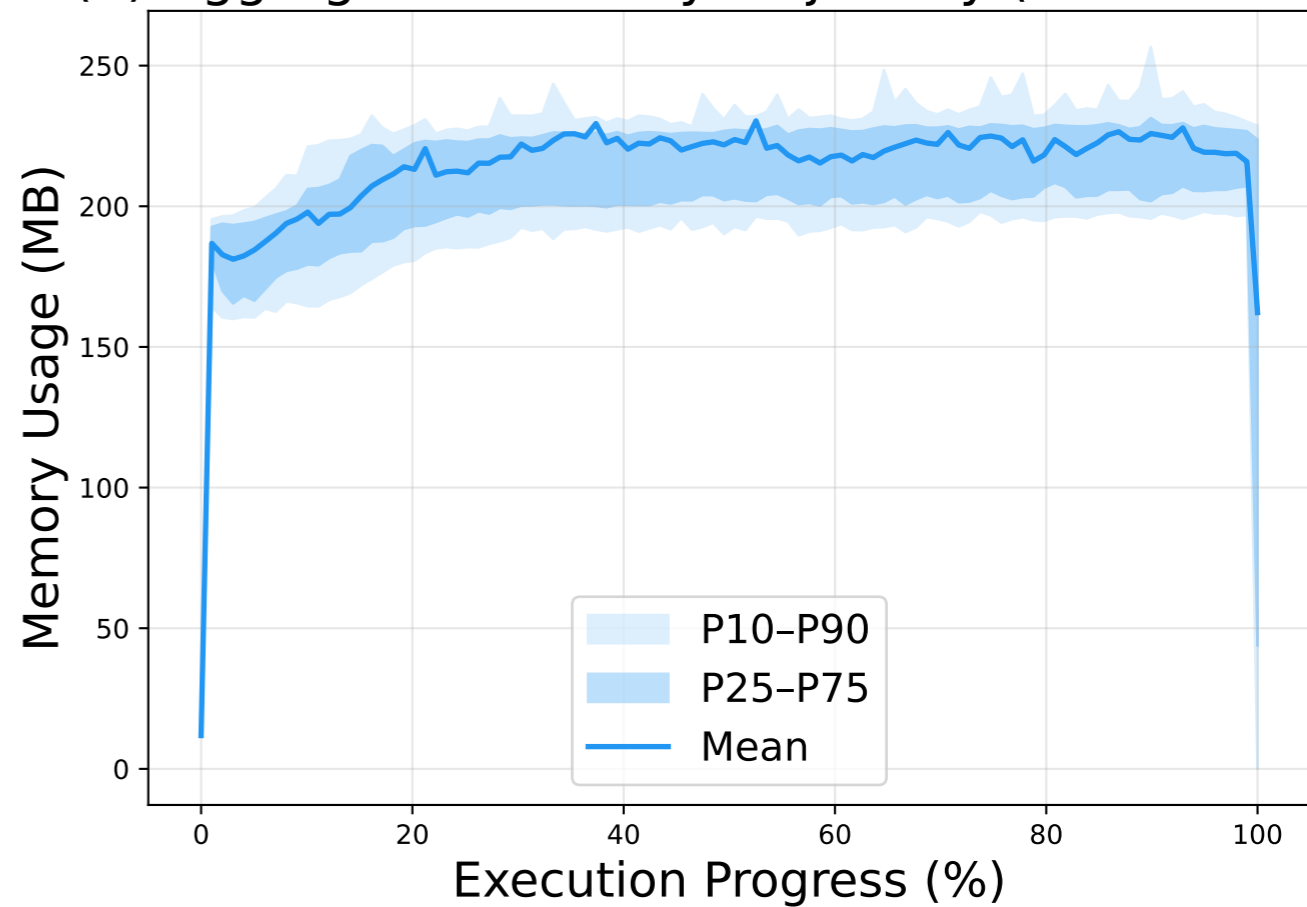
(b) Aggregated Memory Trajectory (n=114 tasks)
