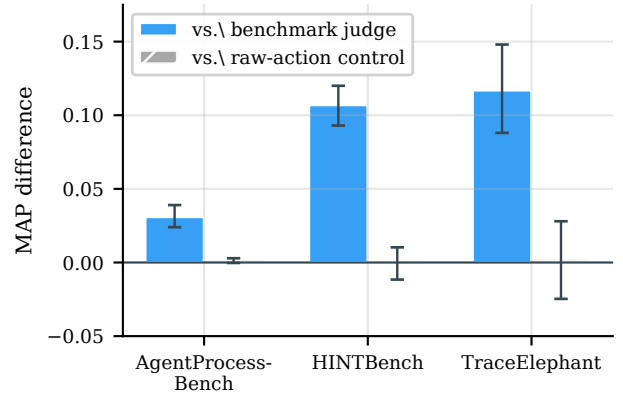
Figure 4: Paired MAP differences with 95% intervals (10,000 resamples). Left: profile improves all three benchmarks (intervals above zero). Right: semantic vs raw-action ablation indistinguishable (intervals span zero).
