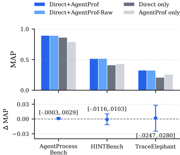
Figure 4: MAP over the complete RQ2 populations (614, 400, and 220 labeled queries). AGENTPROF-Raw ablates only AGENTPROF’s semantic prefix. Higher is better.
