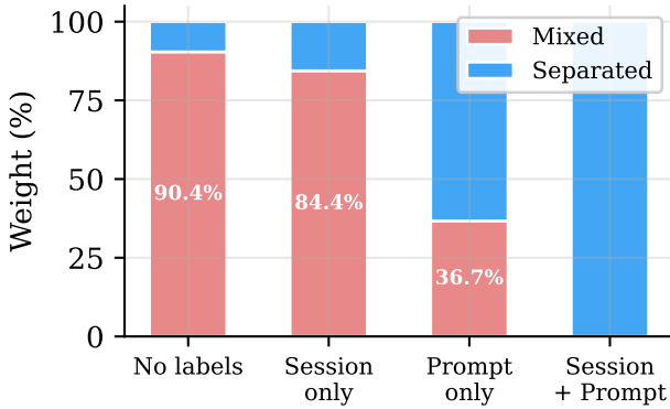
Figure 2: RQ1: Semantic-axis ablation on 183,714 system observations. Adding prompt labels reduces mixed weight from 90.4% to 36.7%. Session labels alone barely help (84.4%).
