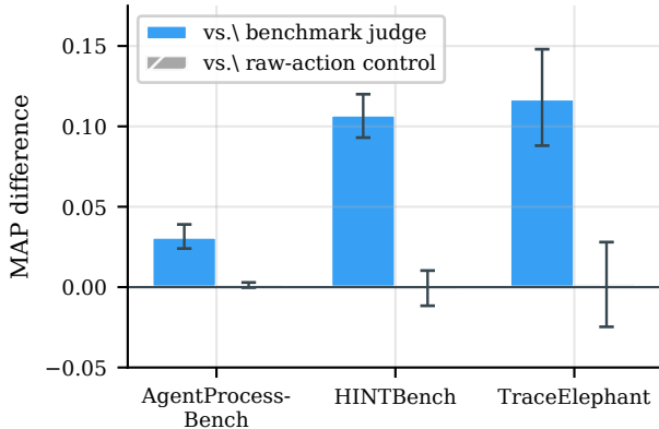
Figure 6: Paired MAP differences with 95% confidence intervals from 10,000 bootstrap resamples. Adding the profile (constructed without seeing fault labels) to each benchmark’s own diagnostic improves ranking on all three workloads (left bars above zero), whereas the semantic names and raw-action ablation are indistinguishable (right bars span zero). Grouping plus retained evidence, not the names, drives this gain.
