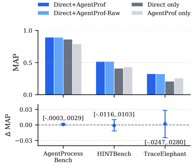
Figure 4: MAP over the complete RQ2 populations (614, 400, and 220 labeled queries). AGENTPROF-Raw ablates only AGENTPROF’s semantic prefix. Higher is better.
