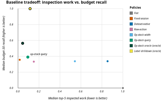
Figure 3: RQ2: Inspection work vs. budget-30 recall across policies. Op-stack query-aware (labeled) achieves low work (0.094) with moderate recall (0.39), while flat requires full inspection and fixed-session fragments into 285 groups. Oracle policies (large dots) are upper bounds.
