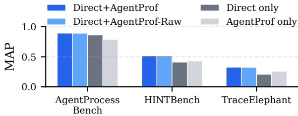
Figure 4: MAP over the complete RQ2 populations (614, 400, and 220 labeled queries). AGENTPROF-Raw ablates only AGENTPROF’s semantic prefix. Higher is better.
