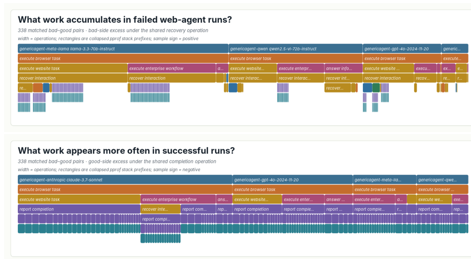
Figure 5: One signed profile over all 338 bad-good pairs, read from both sides. The signed profile is the difference of two nonnegative profiles, bad minus good, which stock pprof renders as positive and negative sample values. Top : positive samples under recover interaction, 3,286 bad-side versus 455 good-side occurrences. Bottom : negative samples under report completion , 135 bad-side versus 191 good-side occurrences. These are aggregate diagnostic differences, not causal effects.
