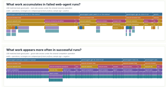
Figure 3: One signed profile over all 338 bad–good pairs, read from both sides. The signed profile is the difference of two nonnegative profiles, bad minus good, which stock pprof renders as positive and negative sample values. Top : positive samples under recover interaction, 3,286 bad-side versus 455 good-side occurrences. Bottom : negative samples under report completion , 135 bad-side versus 191 good-side occurrences. These are aggregate diagnostic differences, not causal effects.
