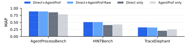
Figure 4: MAP over the complete RQ2 populations (614, 400, and 220 labeled queries). AGENTPROF-Raw ablates only AGENTPROF’s semantic prefix. Higher is better.
