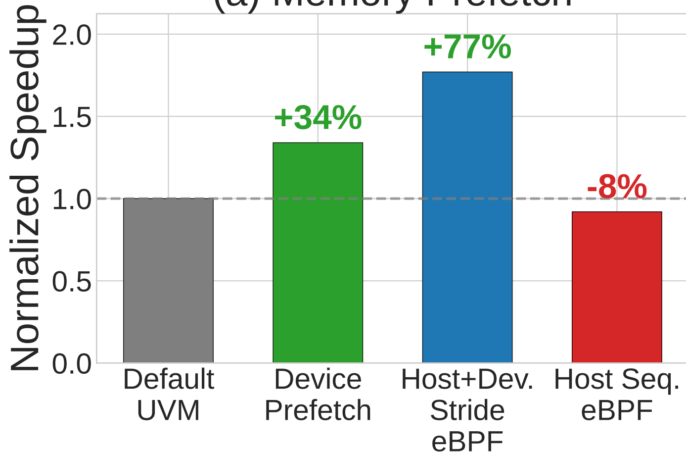
(a) Memory Prefetch
