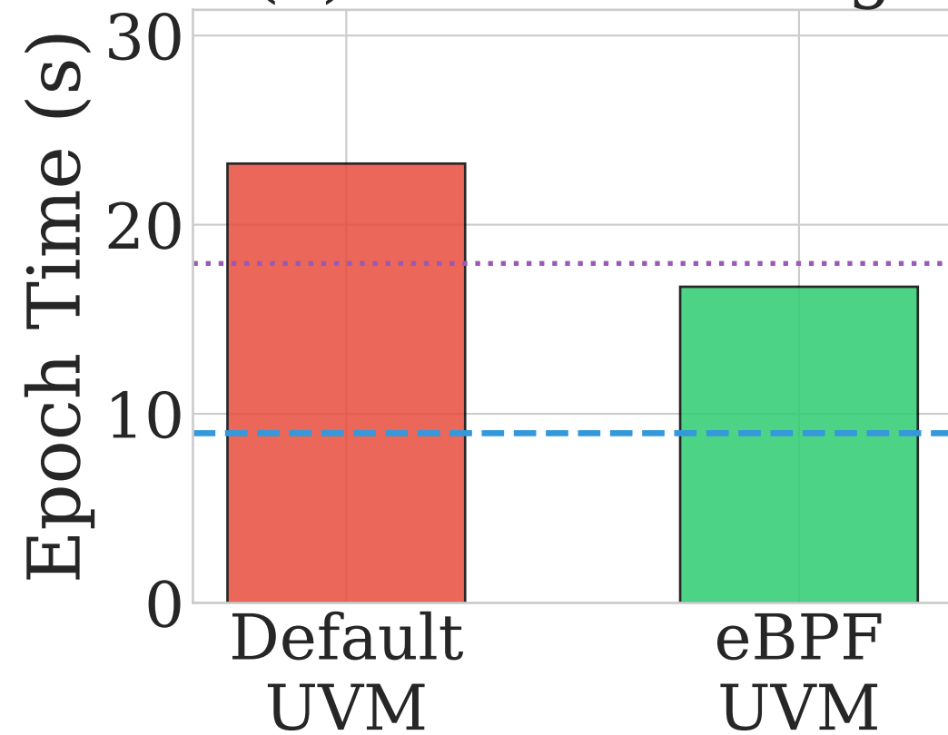
(c) GNN Training
