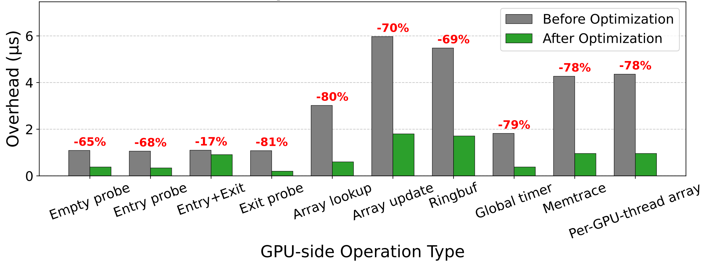
(a) GPU-side Operations (Overhead vs Baseline)
