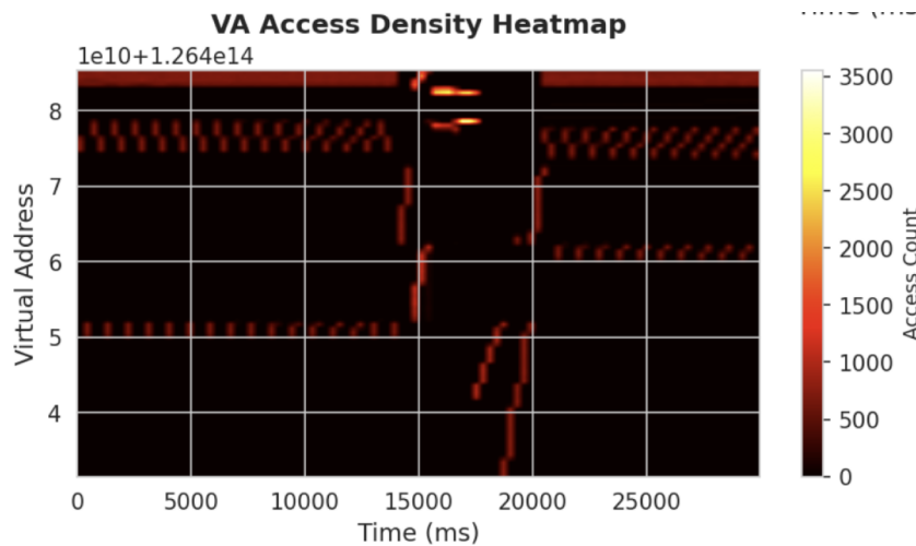
PyTorch DNN Training
