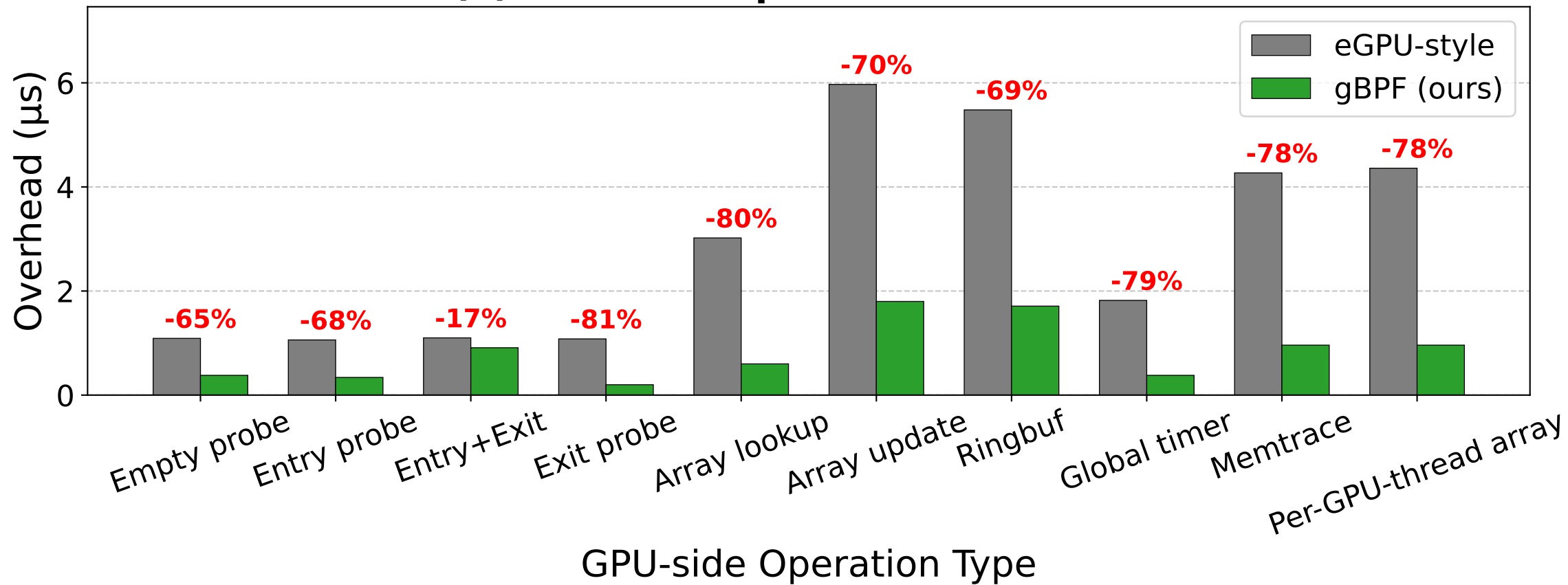
(a) GPU-side Operations Overhead
