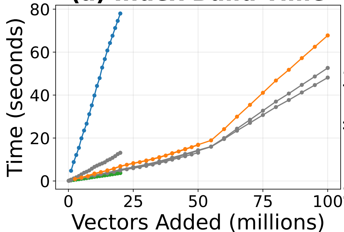
(a) Index Build Time
