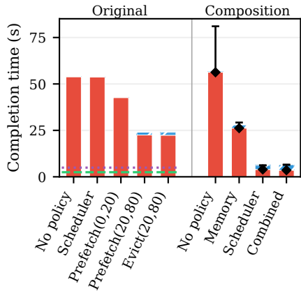
(a) HotSpot
