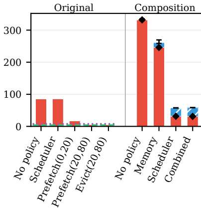
(c) K-Means
