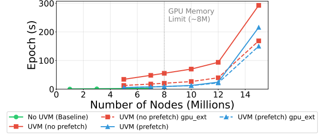
Figure 10. GCN training epoch time vs graph size on PyTorch.
