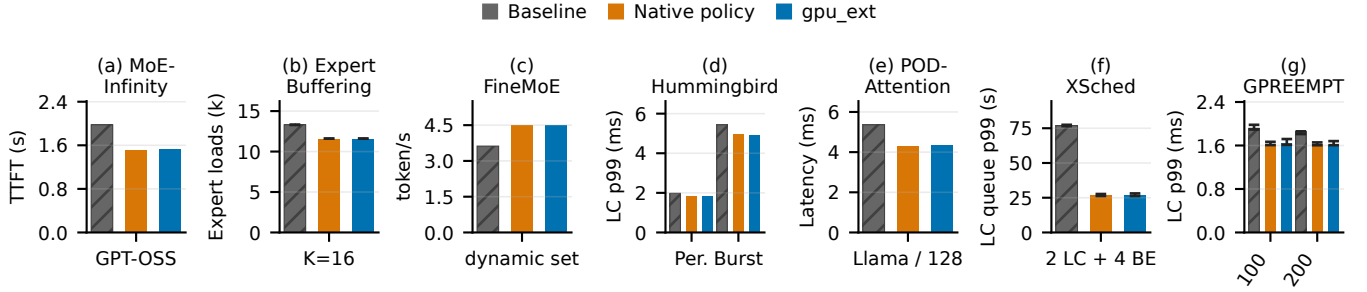
Figure 15. Policy comparisons. Baselines are (a) prediction-disabled expert caching, (b) fixed-K FIFO, (c) prefetching all positively predicted experts, (d,g) default scheduling, (e) two-stream FlashAttention, and (f) native CUDA. In (d), Per. and Burst denote periodic and BurstGPT arrivals. Panel (e) uses Llama decode batch 128. Bars show medians, whiskers show full ranges. Panel (g) uses VGG19 LC at 100 requests/s with ResNet152 BE at 100 or 200 requests/s.
