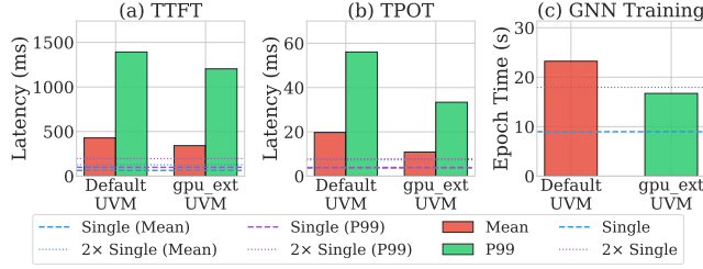
Figure 13. Two-tenant co-location: llama.cpp inference (LC) + GNN training (BE).
