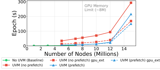
Figure 10. GCN training epoch time vs graph size on PyTorch.
