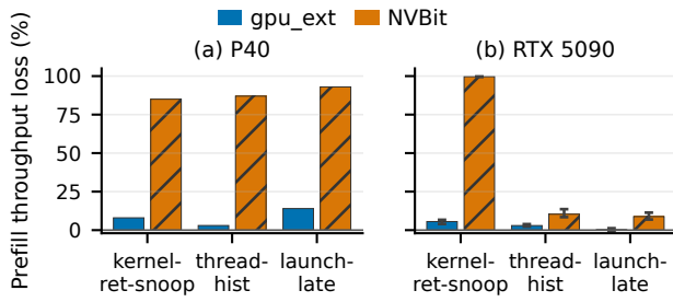
Figure 16. Prefill throughput loss relative to an uninstrumented baseline. (a) P40, Llama 1B. (b) RTX 5090, TinyLlama-1.1B.
