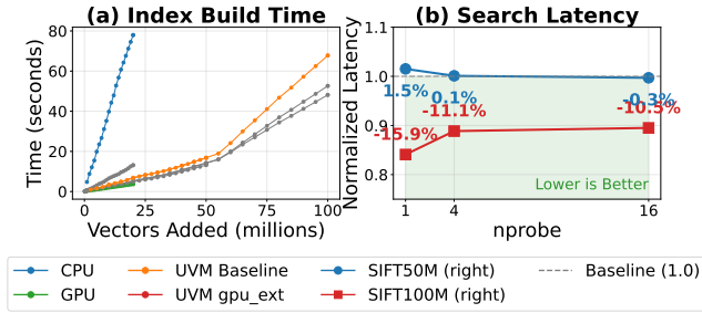
Figure 11. Faiss index build time and search latency normalized to default UVM under oversubscription.
