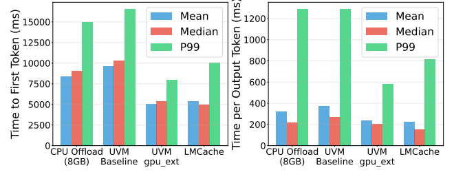
Figure 9. Time-to-first-token and time per output token on Qwen-30B MoE inference with vLLM.
