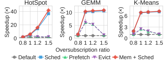
Figure 12. High-priority completion speedup over Default as the oversubscription ratio increases. Points show medians of five paired speedups, and whiskers show their ranges.
