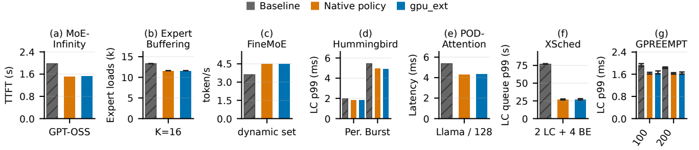
Figure 15. Policy comparisons. Baselines are (a) prediction-disabled expert caching, (b) fixed- K FIFO, (c) prefetching all positively predicted experts, (d,g) default scheduling, (e) two-stream FlashAttention, and (f) native CUDA. In (d), Per. and Burst denote periodic and BurstGPT arrivals. Panel (e) uses Llama decode batch 128. Bars show medians, whiskers show full ranges. Panel (g) uses VGG19 LC at 100 requests/s with ResNet152 BE at 100 or 200 requests/s.
