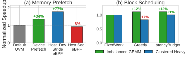
Figure 7. Single-tenant policy evaluation (normalized speedup, higher is better): (a) memory prefetch policies on vector-add; (b) block scheduling policies on GEMM.
