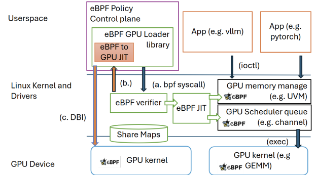
Figure 4. gpu_ext architecture. (a) eBPF syscall deploys policies to verifier and driver hooks; (b) GPU JIT after verification; (c) DBI injects trampolines into GPU kernels.
