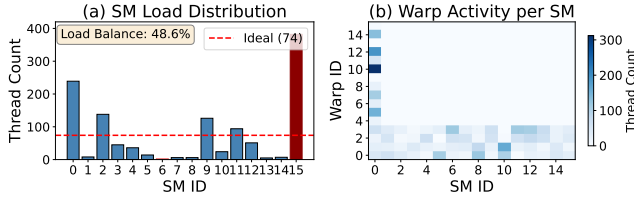
Figure 3. GPU thread scheduling imbalance observed via eBPF tracing. (a) SM load distribution: 127 \times imbalance. (b) Warp activity heatmap across SMs.
