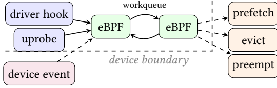
Figure 5. Policy execution model: CPU eBPF policies vs gpu_ext.
