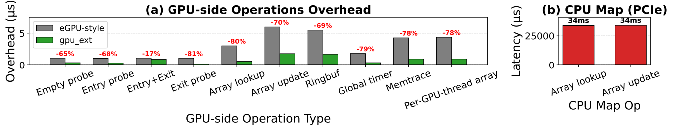
Figure 14. Device-side overhead. (a) Naive per-thread injection vs gpu_ext 's SIMT-aware execution. (b) CPU map access latency via PCIe vs GPU-side operations.
