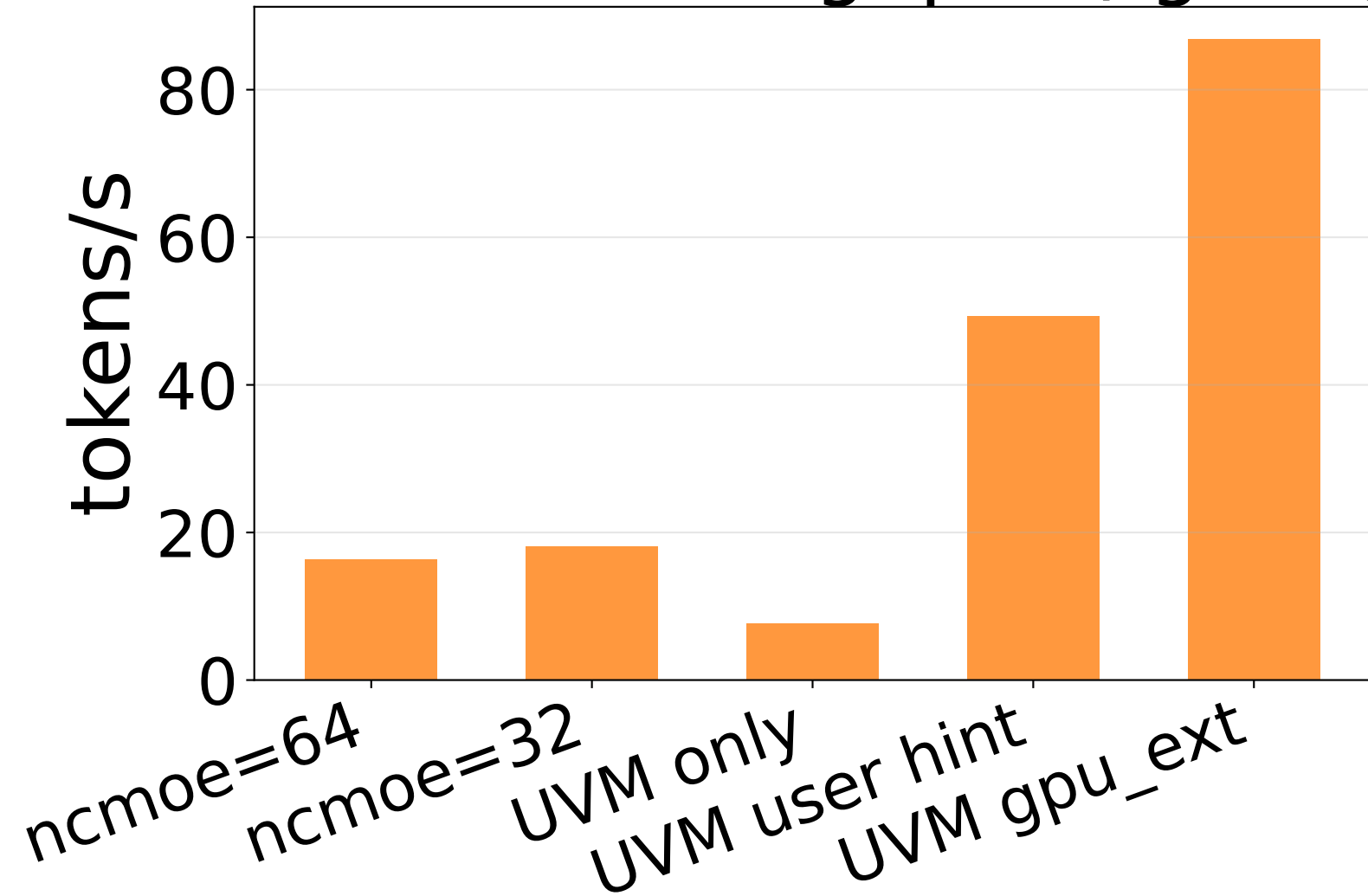
Decode Throughput (tg128)
