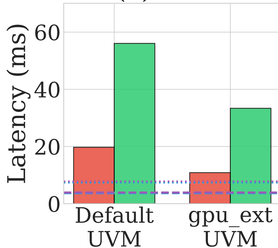
(b) TPOT
