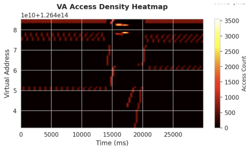
PyTorch DNN Training
