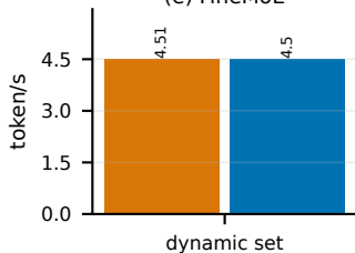
(e) FineMoE
