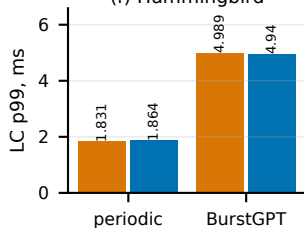
(f) Hummingbird
