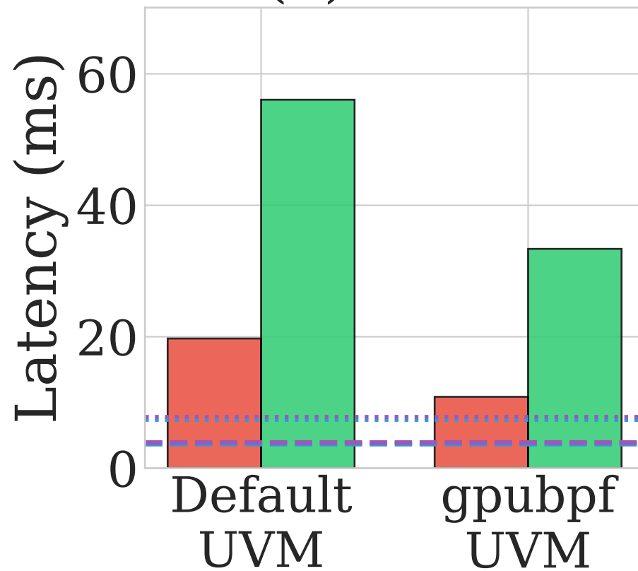
(b) TPOT
