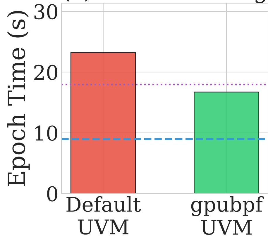
(c) GNN Training
