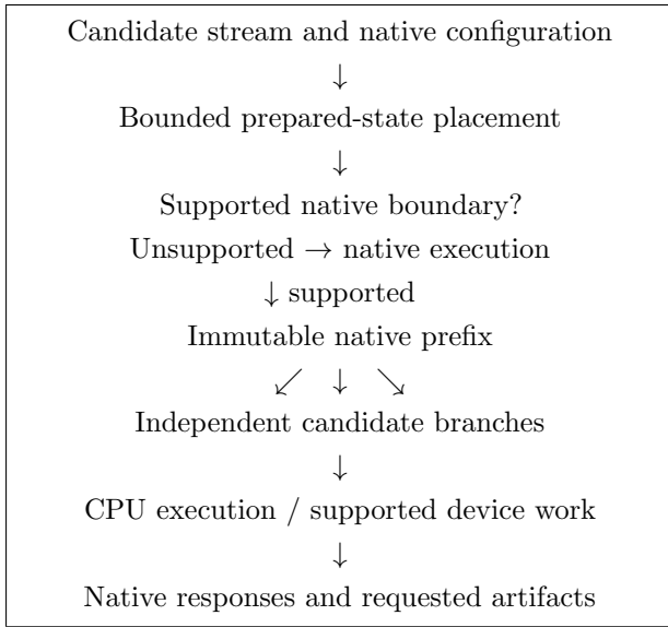
Figure 1: A prepared parent performs no candidate verification. Disposable branches retain the prefix’s preparation while separating candidate histories and lifetimes.
