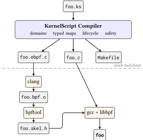
Figure 1. Compilation pipeline. The compiler checks cross-boundary invariants and emits C; the stock clang/bpftool/libbpf toolchain produces the final binary.
