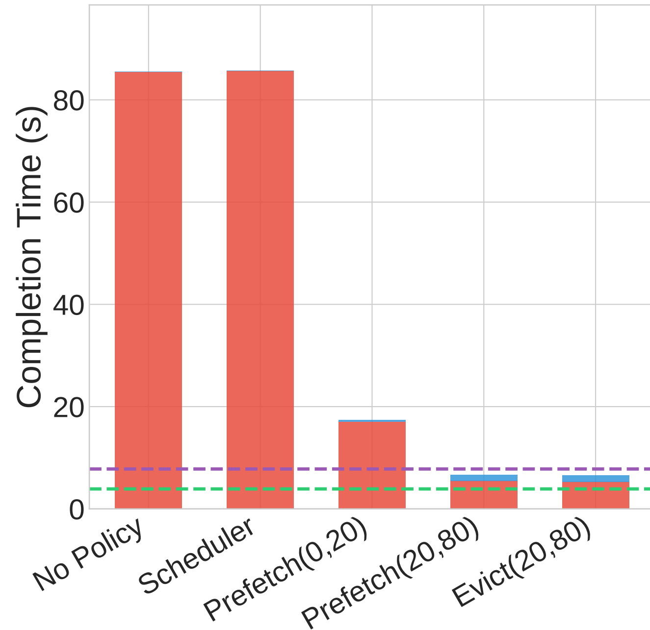
K-Means
