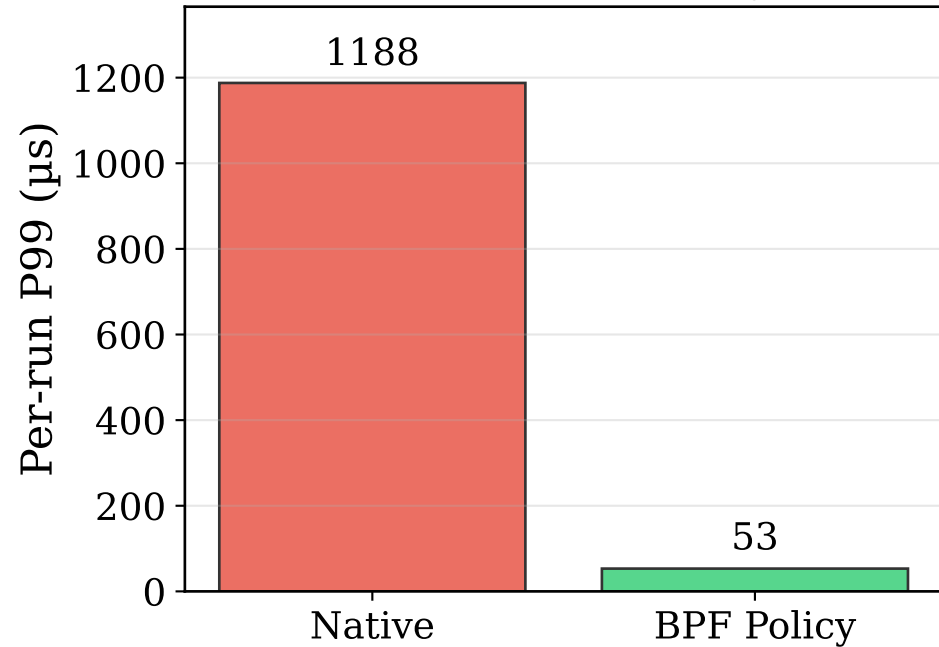
(a) LC P99 Launch Latency [-96%]
