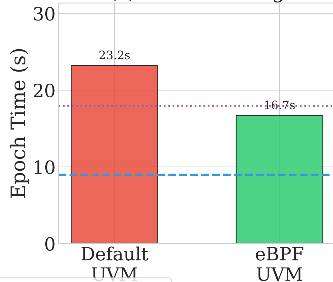
(c) GNN Training
