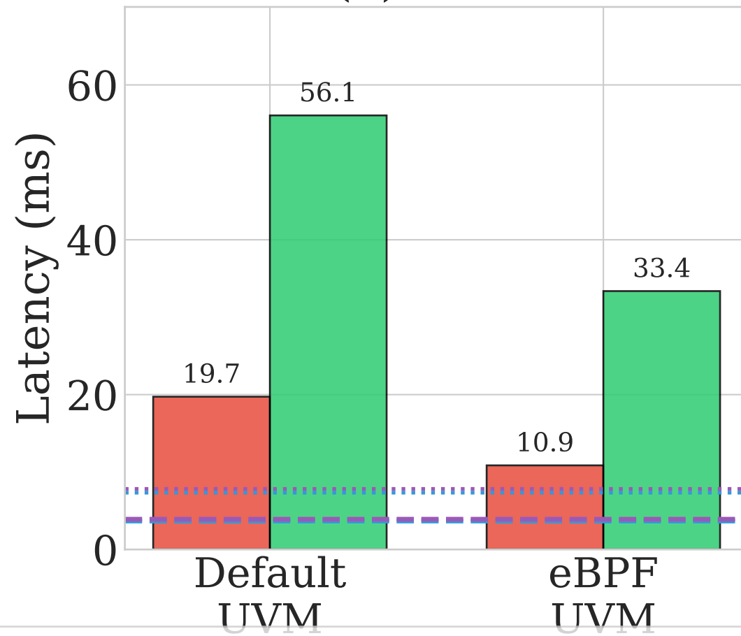
(b) TPOT
