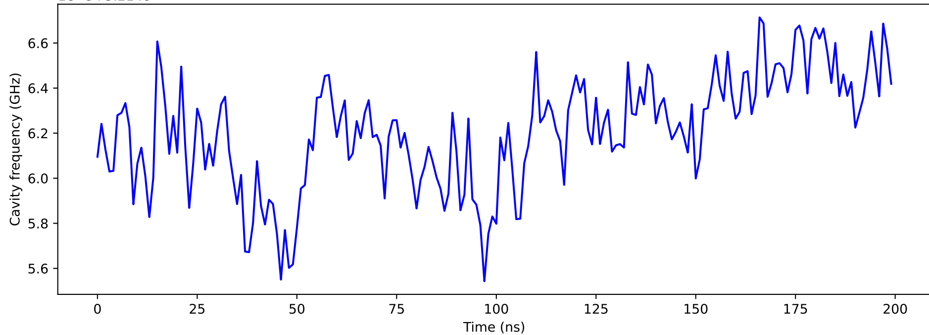
Cavity frequency fluctuation due to 1/f flux noise
