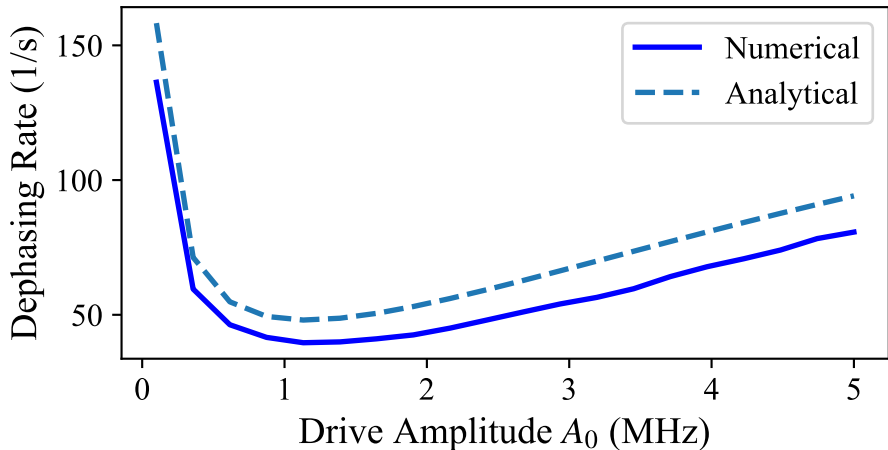
Dephasing Rate vs Drive Amplitude
