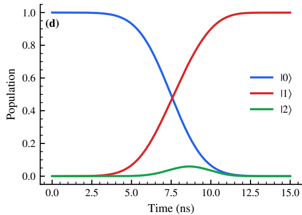
with DRAG ( \delta/2\pi = 0.005 GHz, \lambda = 0.79 )
