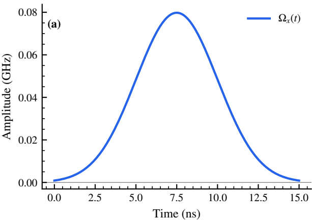
Control — with DRAG
