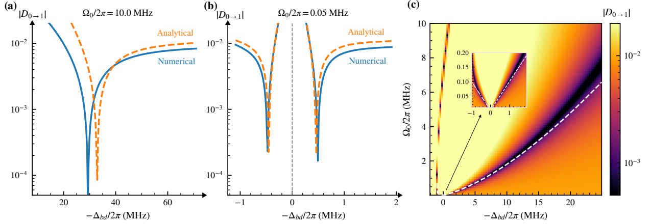
Figure 7.1: Drive-induced flux sweet spots, defined by D_{0 \rightarrow 1} = 0 . (a) Unselective regime at \Omega_0/2\pi = 10 MHz, showing a single sweet spot. (b) Selective regime at \Omega_0/2\pi = 0.05 MHz, showing two symmetric sweet spots about the effective resonance. (c) Two-dimensional map of D_{0 \rightarrow 1} versus drive amplitude \Omega_0 and detuning \Delta_{bd} ; Dashed curves denote analytical sweet-spot conditions from Eqs. (7.51) and (7.58) for the main panel and the inset, respectively.
