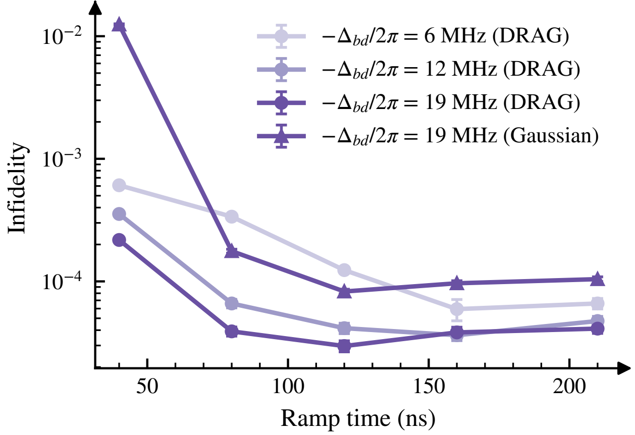
Figure 7.4: State-preparation infidelity \mathcal{I}(\tau) versus ramp time \tau for several detunings \Delta_{bd} , comparing Gaussian and DRAG ramps. The non-monotonic dependence reflects the trade-off between coherent leakage from unwanted transitions (suppressed for longer \tau ) and decoherence (which accumulates for longer \tau ).
