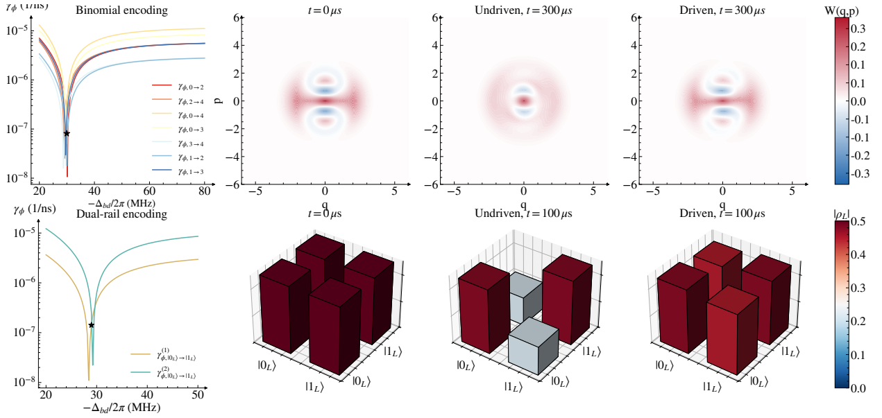
Figure 9.1: Driven sweet-spot protection for bosonic encodings ( \Omega_0/2\pi = 10 MHz throughout). Binomial code — (a) Dephasing rate \gamma_{\phi,n \rightarrow m} of cavity transitions due to FTT-frequency fluctuations as a function of \Delta_{bd} ; the star marks \Delta_{bd}/2\pi = -30 MHz, where all relevant \gamma_{\phi,n \rightarrow m} are suppressed by at least \sim 13\times . (b) Wigner function of |+_L\rangle at t = 300 \mu\text{s} : the driven case retains the interference fringes that are lost without the drive. Dual-rail encoding — (c) Dephasing rate \gamma_{\phi,0 \rightarrow 1}^{(i)} for each cavity as a function of \Delta_{bd} ; both cavities exhibit \sim 10\times lower dephasing near -\Delta_{bd}/2\pi \sim 29 MHz. (d) Logical-subspace tomography for one dual-rail qubit: the drive suppresses dephasing, while leakage from single-photon loss remains unchanged.
