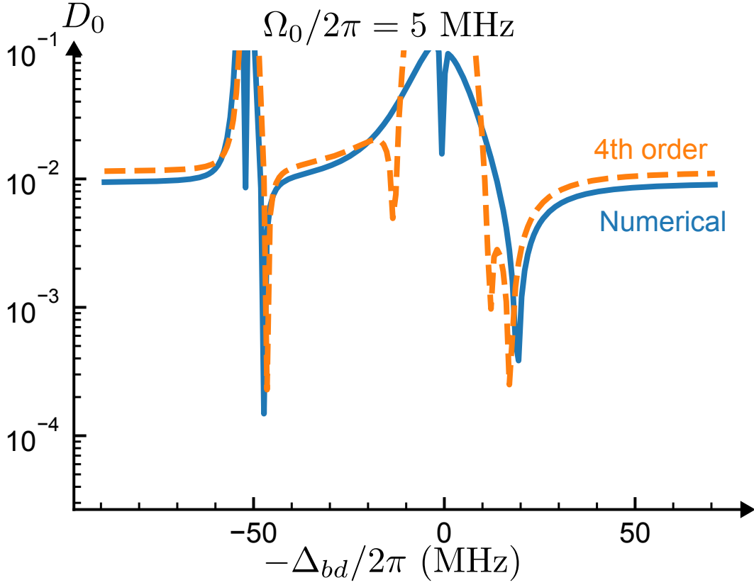
Figure 7.2: Susceptibility D_0 including higher-order corrections in the Schrieffer–Wolff expansion. An additional sweet spot appears near -\Delta_{bd} \simeq K/2 , arising from hybridization between |g\rangle and |f\rangle states
