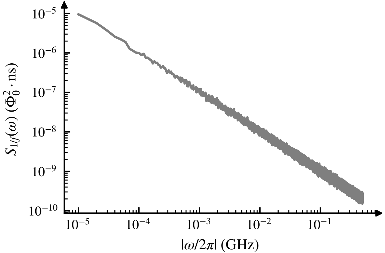
Figure 8.1: Power spectral density of \delta\Phi(t) for 100 representative 1/f noise trajectories generated with the cutoffs specified below.
