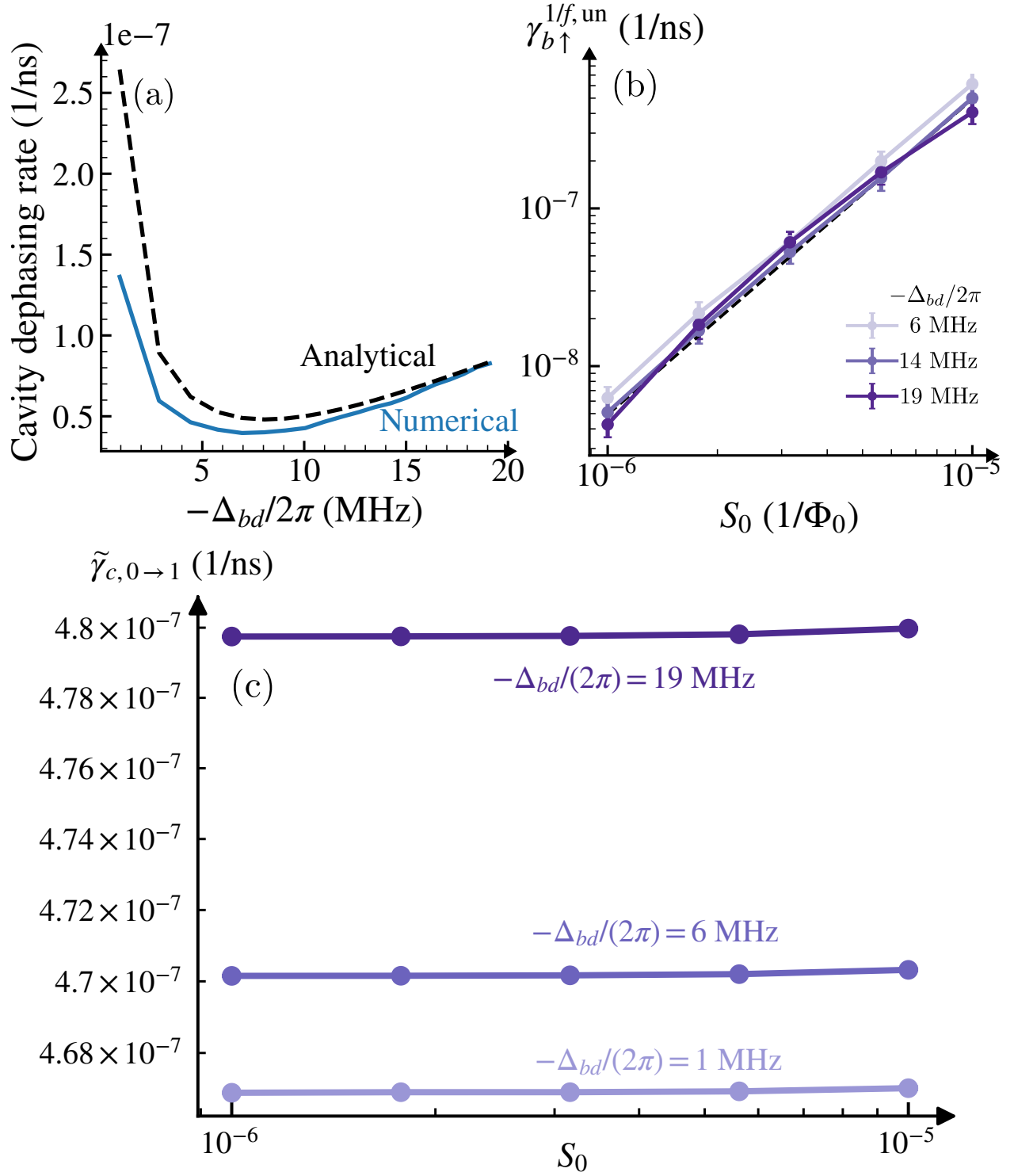
Figure 8.2: Numerical validation of rates in the unselective regime. (a) Reference dephasing rate \gamma_{b\uparrow}^{\text{un}} + \gamma_{c\phi}^{\text{un}} extracted from Monte Carlo simulations with \delta\Phi(t) = 0 , compared with the analytical approximation in Eq. (8.34). (b) Flux-noise-induced depolarization rate \gamma_{b\uparrow}^{1/f, \text{un}} versus noise amplitude S_0 . The quadratic scaling in S_0 and agreement with \gamma_{b\uparrow}^{1/f, \text{un}} = \left(\frac{\partial \omega_b}{\partial \Phi}\right)^2 \frac{S_0^2}{4K} (black dashed line) are observed. (c) Cavity decay rate with sweet-spot drive.
