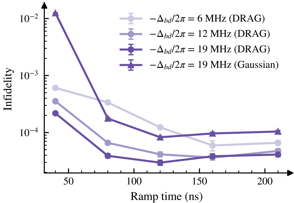
Figure 7.3: State-preparation infidelity \mathcal{I}(\tau) versus ramp time \tau for several detunings \Delta_{bd} , comparing Gaussian and DRAG ramps. The non-monotonic dependence reflects the trade-off between coherent leakage from unwanted transitions (suppressed for longer \tau ) and decoherence (which accumulates for longer \tau ).
