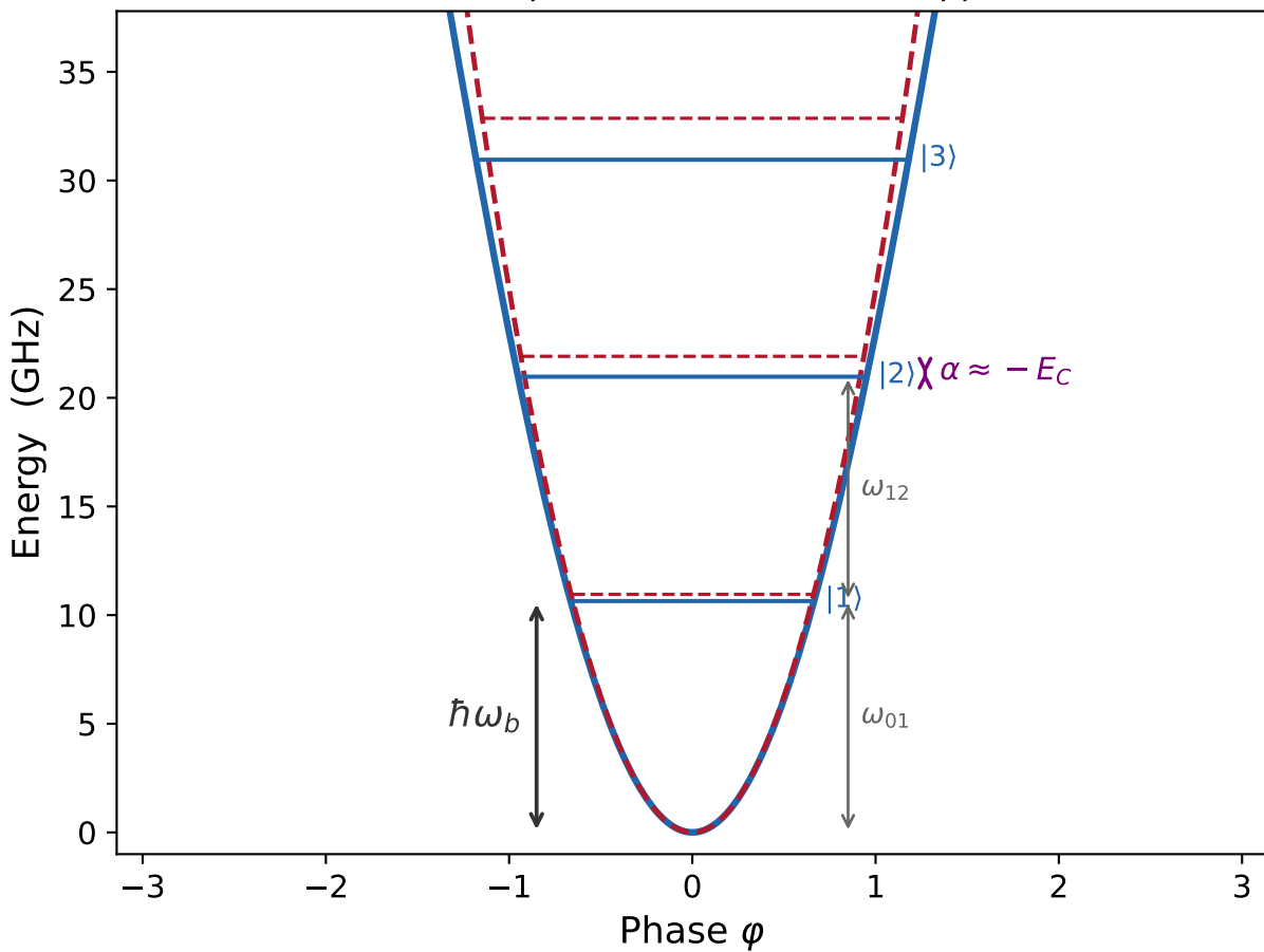
Transmon: cosine potential vs. harmonic approximation
