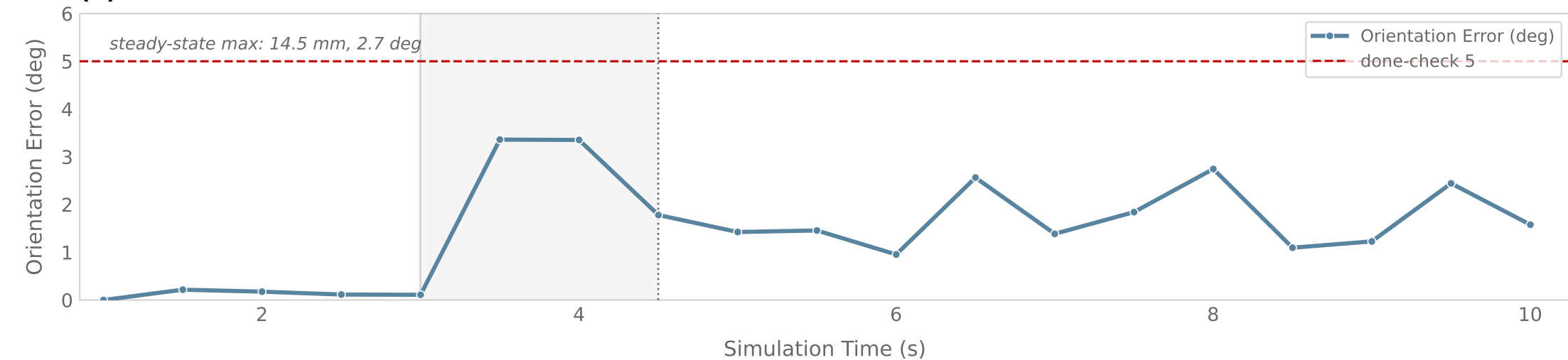
(b) Orientation Hold Error
