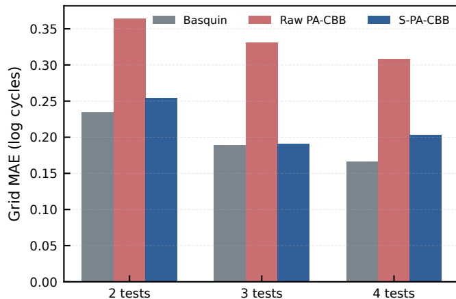
(b) Selective mean correction
