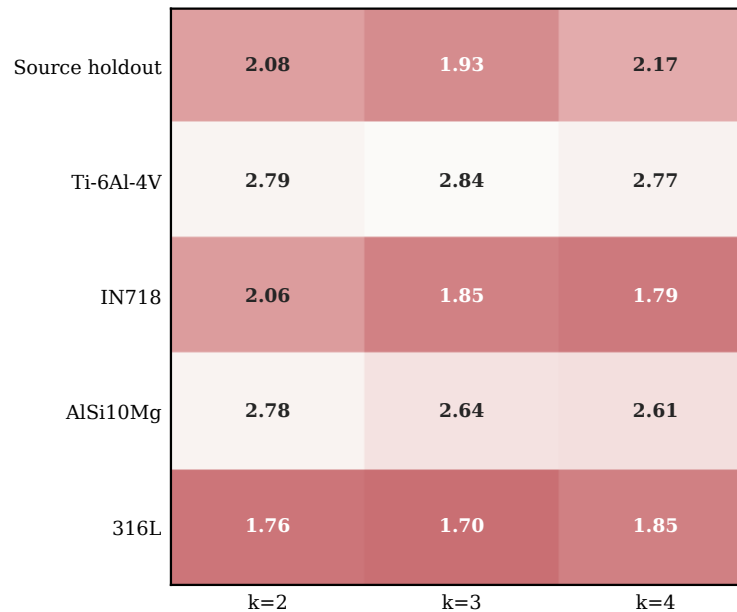
Pointwise interval score
