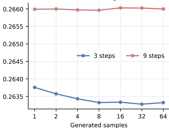
Raw 90% coverage
