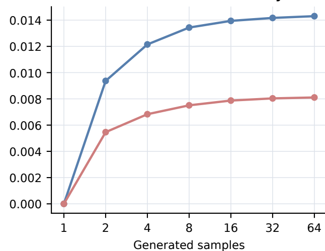
Within-ensemble diversity
