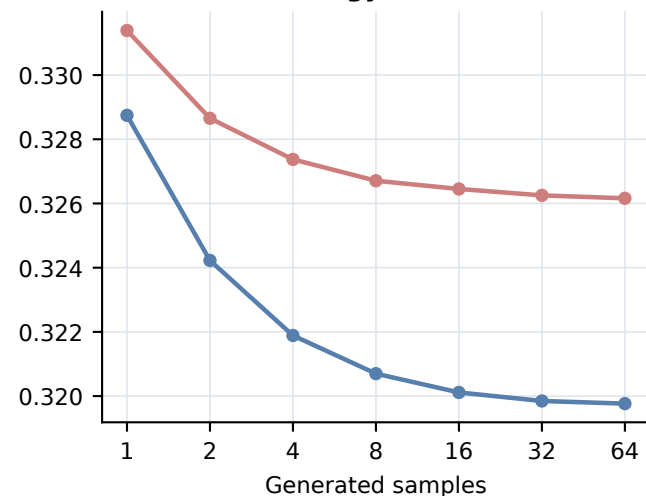
Within-ensemble diversity
