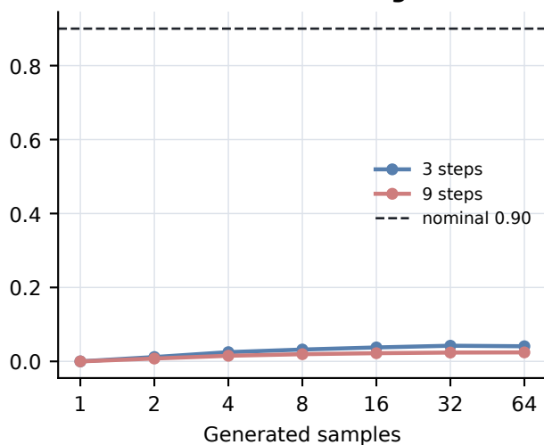
Raw 90% coverage
