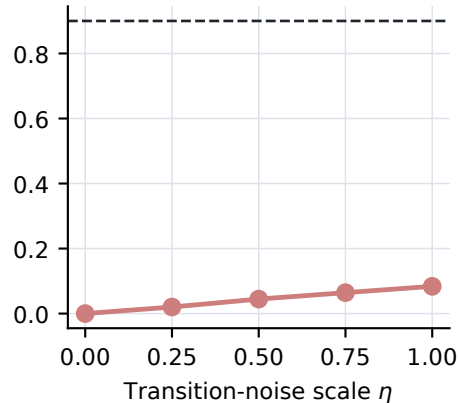
Raw 90% coverage
