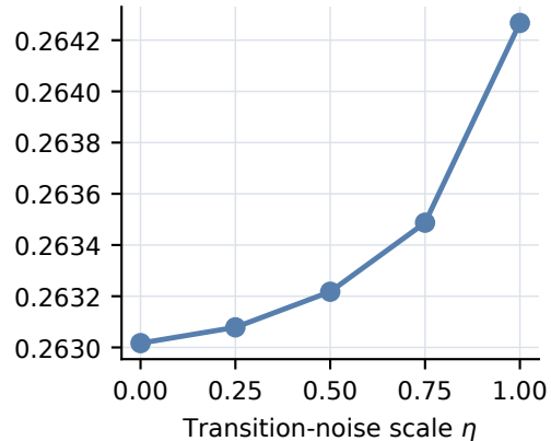
Grid MAE
