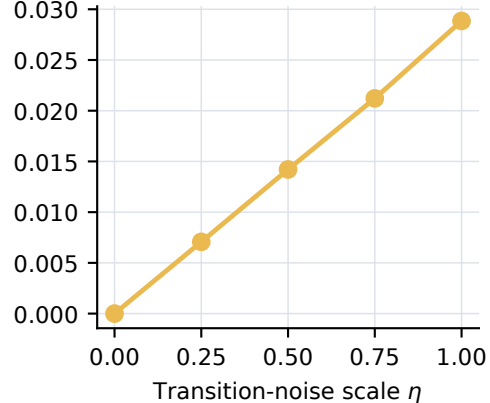
Diversity
