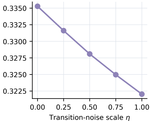
CRPS
