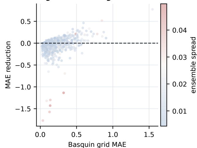
Does generation target hard cases?
