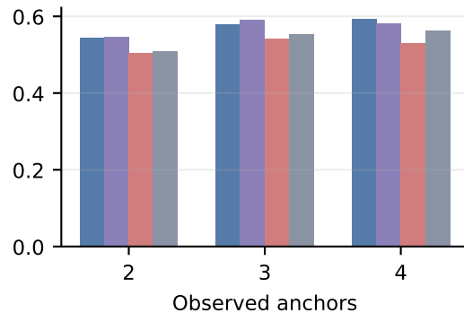
Factor-of-two accuracy
