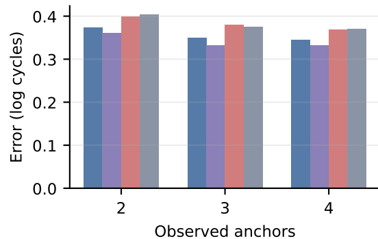
Hidden-point MAE
