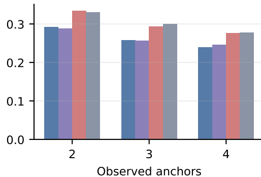
Full-grid MAE
