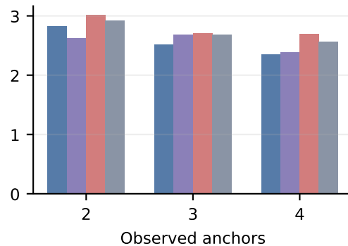
Slope error
