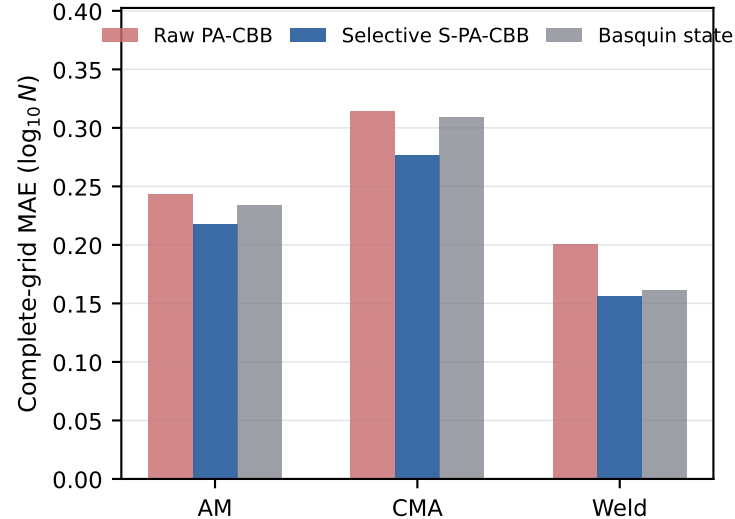
(c) Complete-curve reconstruction at k=4
