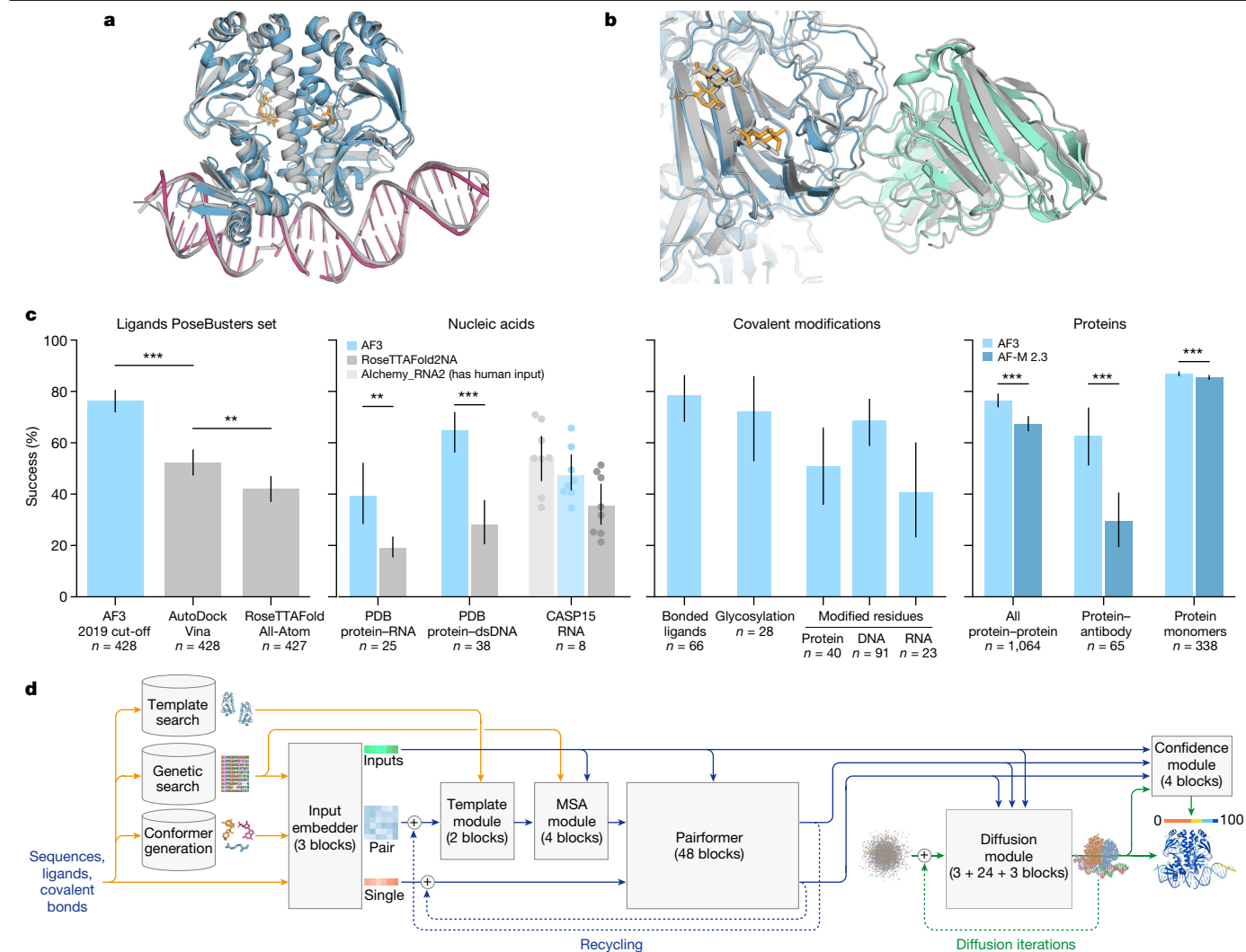
Fig. 1 | AF3 accurately predicts structures across biomolecular complexes.
