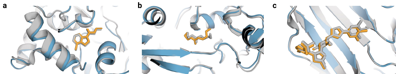
Extended Data Fig. 3 | AlphaFold 3 predictions of PoseBuster examples for which Vina and Gold were inaccurate. Predicted protein chains are shown in blue, predicted ligands in orange, and ground truth in grey. a , Human Notum bound to inhibitor ARUK3004556 (PDB ID 8BTI, ligand RMSD: 0.65 Å).
