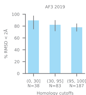
c PoseBusters Version 2
