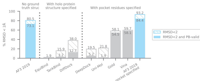
e PoseBusters Version 2
