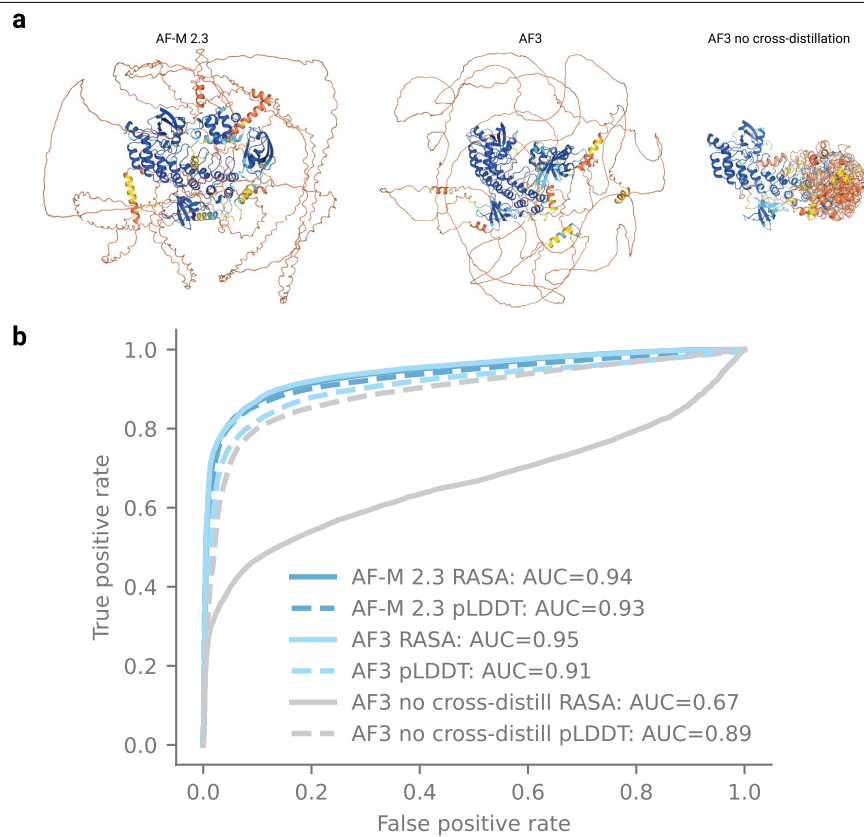
Extended Data Fig. 1 | Disordered region prediction. a , Example prediction for a disordered protein from AlphaFoldMultimer v2.3, AlphaFold 3, and AlphaFold 3 trained without the disordered protein PDB cross distillation set. Protein is DP02376 from the CAID 2 (Critical Assessment of protein Intrinsic Disorder prediction) set. Predictions coloured by pLDDT (orange: pLDDT \leq 50,
